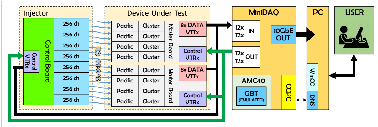
Figure 1: Overall diagram of the Test System
