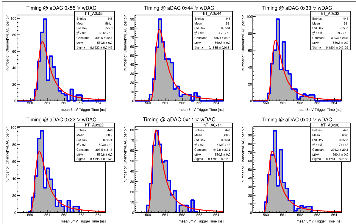
Figure 8: Output pulse timing distribution for multiple pulse amplitude settings.
