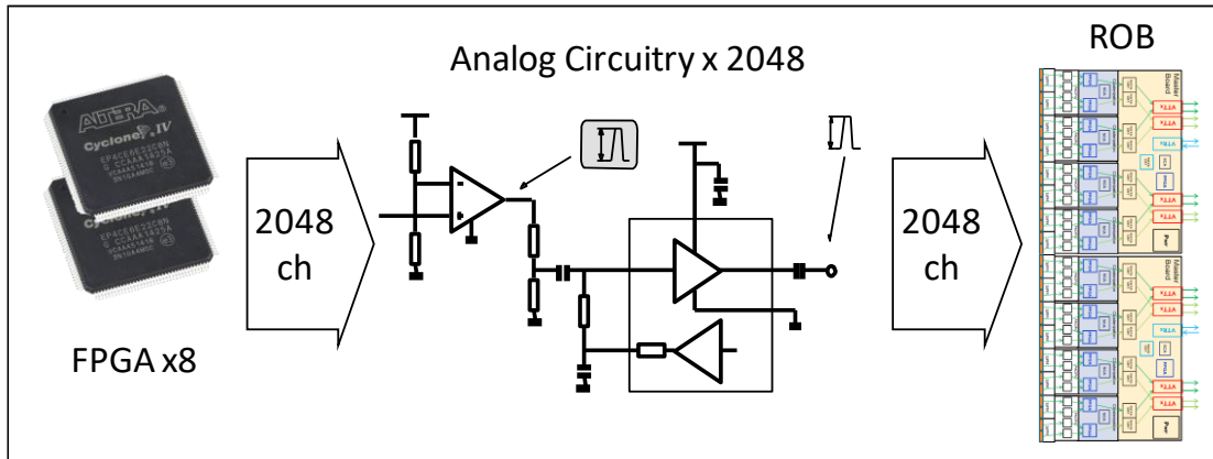
Figure 3: Conceptual diagram of the eight Injector Modules
