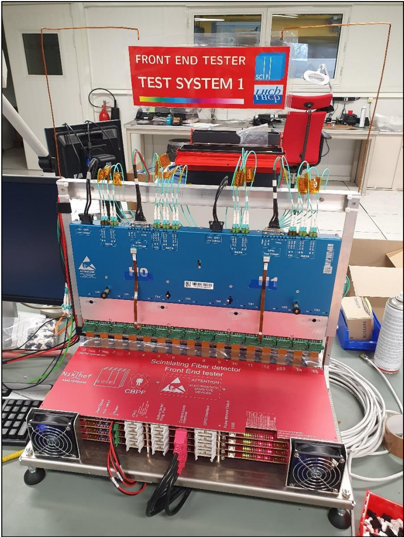
Figure 6: Photo of the fully assembled Test System in operation at LHCb/CERN
