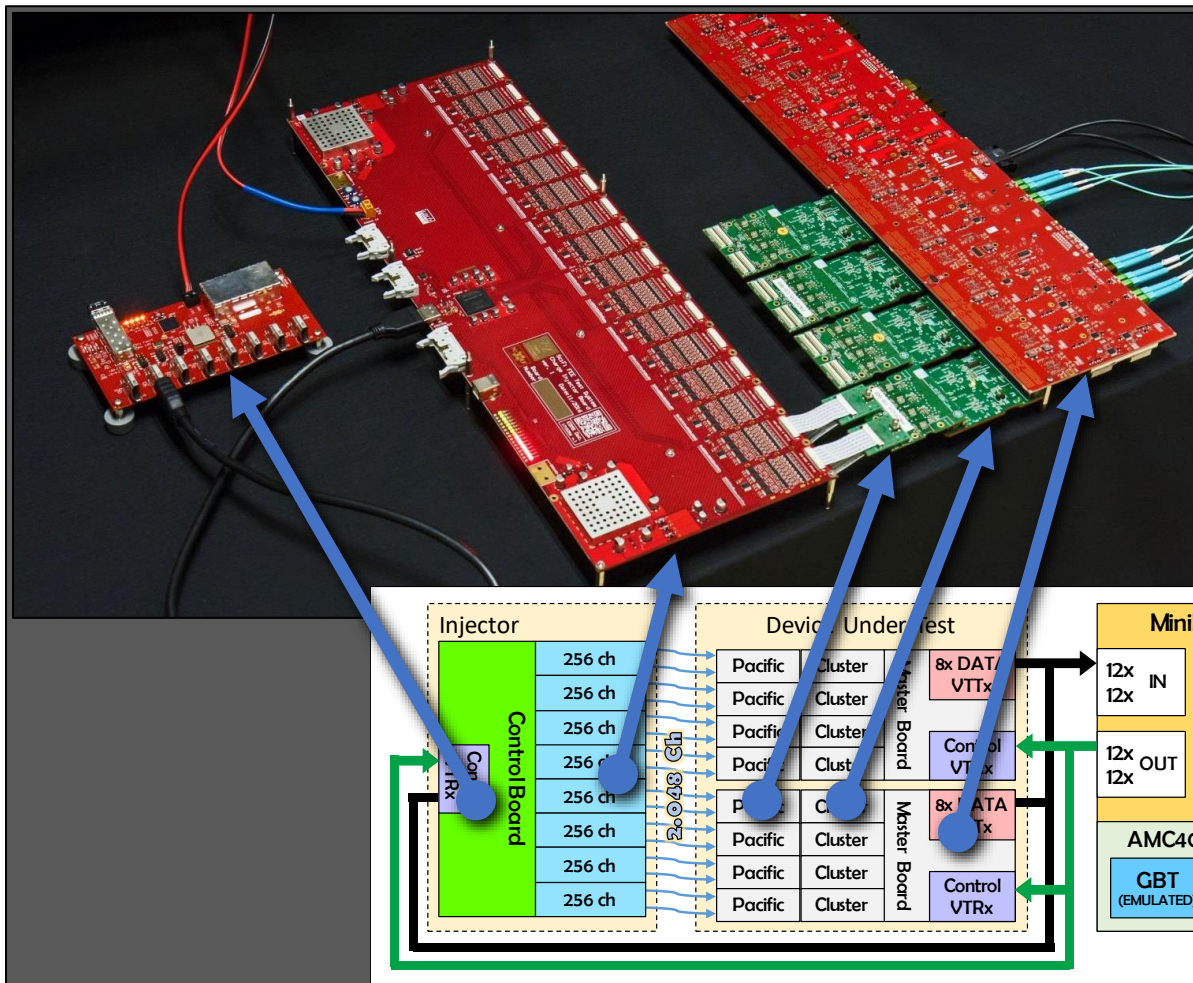
Figure 2: Illustration of the assembled modules in association with the overall diagram
