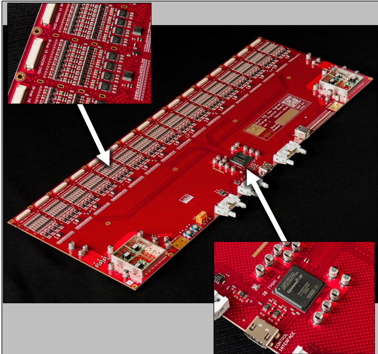
Figure 4: Photo of one of the Injector Modules
