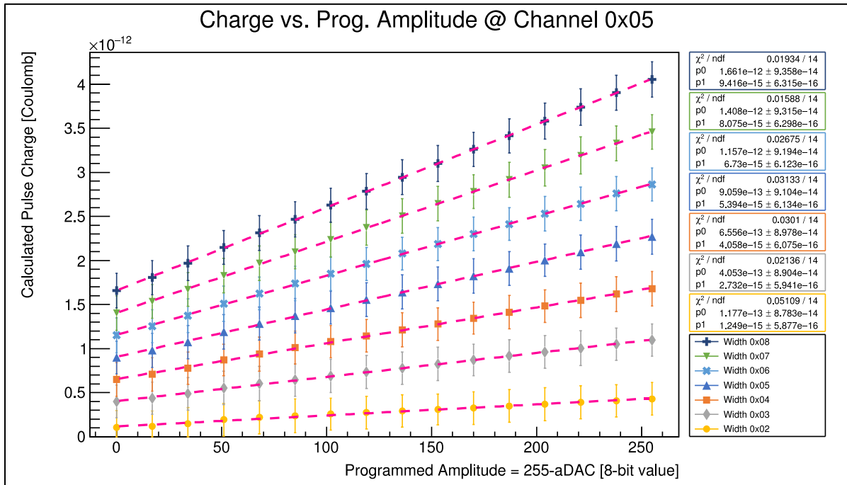
Figure 7: Output Charge calibration curves for multiple pulse width settings.
