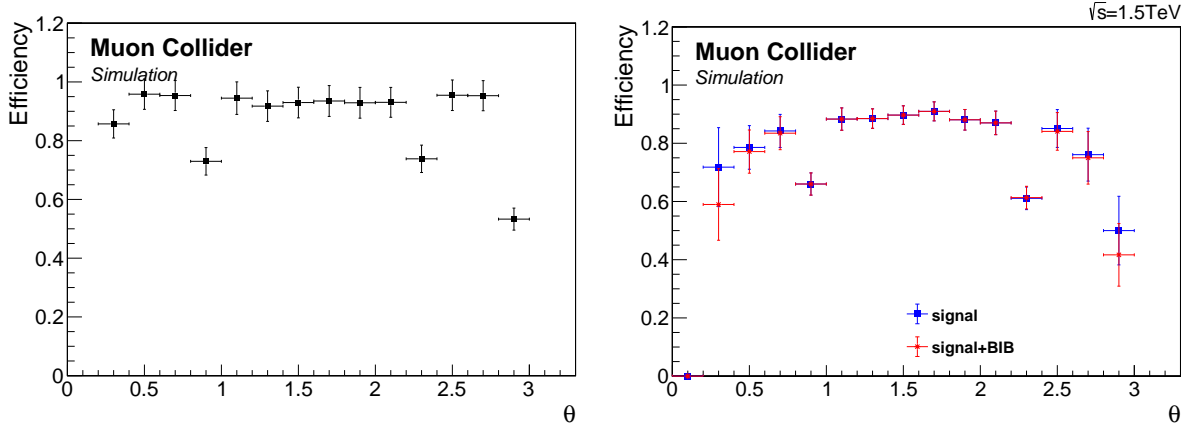
Fig. 42: Muon reconstruction efficiency as a function of the polar angle in a sample of single muons with no BIB overlaid (left) and in a sample with multi-muons in the final state both with and without BIB (right).
