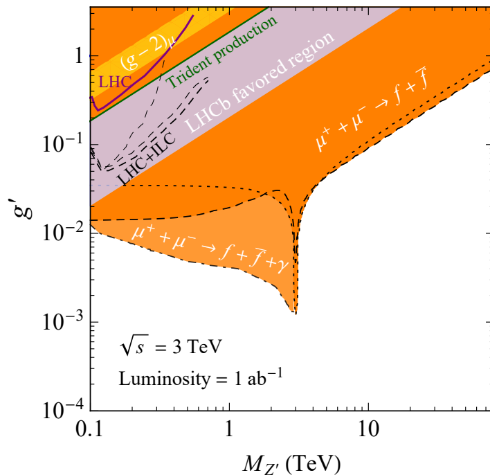
Fig. 22: The sensitivity of the MuC with the COM energy \sqrt{s} = 3 TeV and luminosity L = 1 \text{ ab}^{-1} , given as orange regions. Other limits and projections are also shown for comparison. Our concerned parameter regions explaining the (g-2)_\mu and B anomalies are given as yellow and blue bands, respectively. Figure from Ref. [23].
