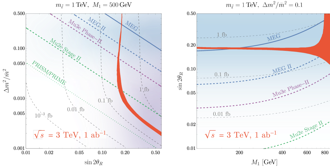
Fig. 21: Constraints on lepton flavor violation in the MSSM in the \Delta m^2/\bar{m}^2 vs. \sin 2\theta_R plane (left) and the \sin 2\theta_R vs. M_1 plane (right) from measurements of the slepton pair production process with flavor-violating final states (red band) at a 3 TeV MuC, assuming 1 \text{ ab}^{-1} of luminosity. The width of the band represents the uncertainty on the reach from the measurement of the slepton and neutralino masses in flavor-conserving channels. The purple and blue shaded lightly shaded regions indicate parameters preferred in Gauge-Mediated Supersymmetry Breaking scenarios and flavor-dependent mediator scenarios, respectively. Both plots assume a mean slepton mass of 1 TeV. In the left plot we fix the neutralino mass M_1 = 500 \text{ GeV} , while in the right figure \Delta m^2/\bar{m}^2 is fixed to 0.1. The current (solid) and expected (dashed, dotted) limits from low-energy lepton flavor violation experiments are indicated by the blue, purple and green lines.
