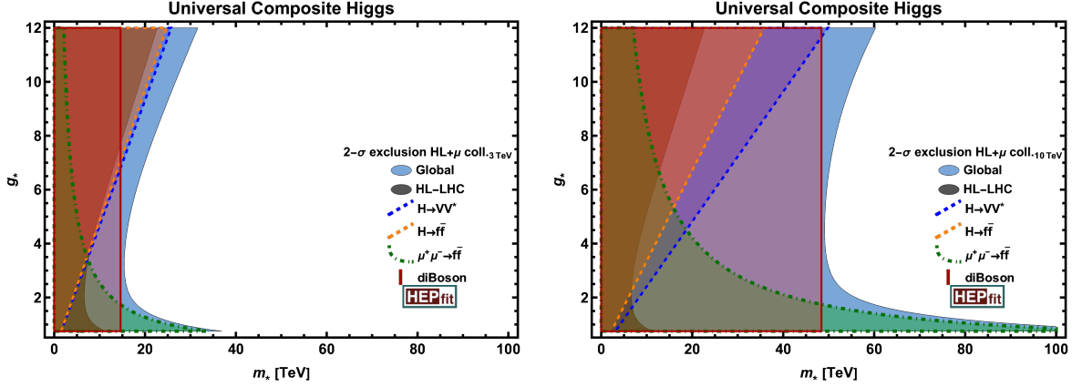
Fig. 5: (Left) 2\text{-}\sigma exclusion regions in the (g_*, m_*) plane from the fit presented in Figure 3, using the SILH power-counting described in Eq. (4) and below (solid regions). The solid and dashed lines denote the contributions to the constraints from different processes. The results correspond to the combination of the HL-LHC with the 3 TeV muon collider. (Right) The same for the 10 TeV muon collider.
