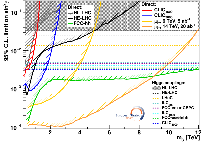
Fig. 6: The direct (solid curves) and indirect (dotted curves) 95 % C.L. reach [59] of heavy singlet mixed with the SM Higgs doublet at various future colliders.
