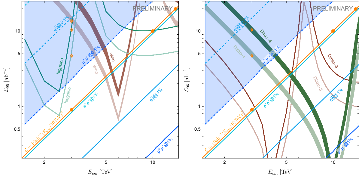
Fig. 11: Minimal luminosity to exclude a thermal pure higgsino or wino dark matter (left panel) a 2.0 TeV Dirac triplet or 4.8 TeV Dirac 4-plet as function of the collider center of mass energy [90] (hyper-charge of the higgsino and Dirac n -plets not taken into account). Lighter color lines are for polarized beams. The thickness of the Wino and Dirac 4-plet bands covers the uncertainty on the thermal mass calculations. Diagonal lines mark the precision at which the total rate of the labeled channels are going to be measured. The shaded area indicates that at least one channel is going to be measured with 0.1% uncertainty and systematic uncertainties need to be evaluated.
