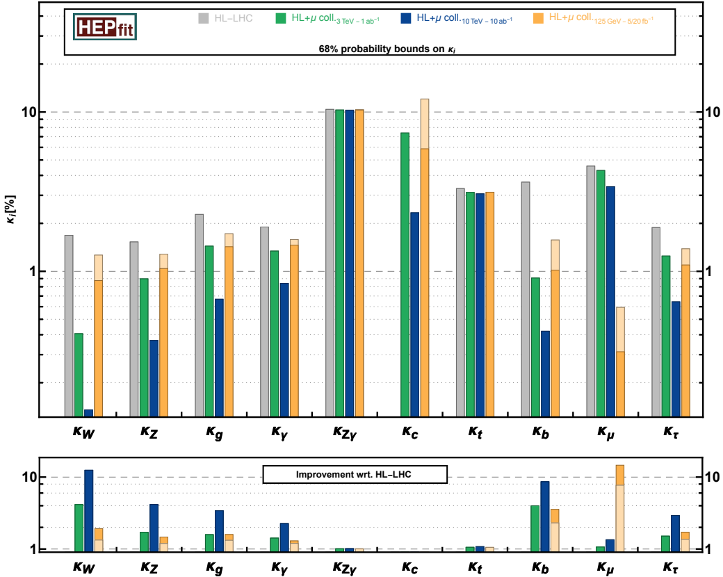
Fig. 2: Sensitivity to modified Higgs couplings in the \kappa framework. We show the marginalized 68% probability reach for each coupling modifier. For the 125 GeV muon collider, light (dark) shades correspond to a luminosity of 5 (20) \text{fb}^{-1} .
