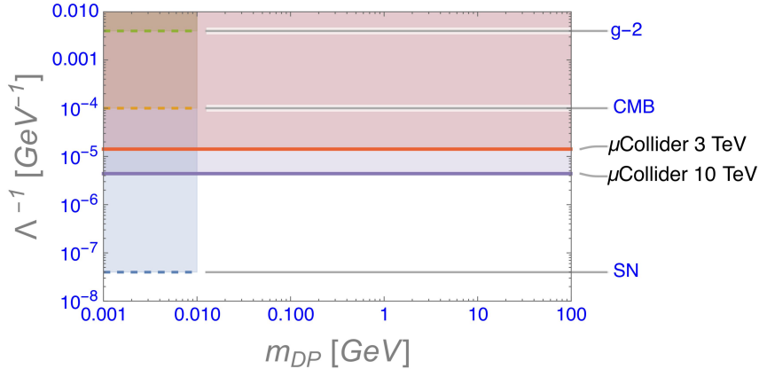
Fig. 27: Limits on 1/\Lambda scale for the dark-photon as a function of the dark-photon mass m_{DP} : for SN the scale of the coupling to muons has been set at 10^{7.4} GeV [212] by the effect of dark radiation on Supernovae dynamics. For CMB see [213]. For g - 2 see [214, 215]. Comparable bounds hold for the ALP to muons because of the similar structure of the interaction vertex. For masses up to 100 GeV the \mu Collider limits are for all practical purposes mass independent.
