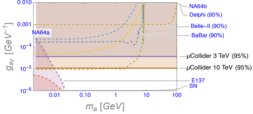
Fig. 28: Limits on g_{a\gamma} = 4/\Lambda as a function of the ALP mass m_a : NA64a [219], Delphi [220] and BaBar [221] are actual limits. Belle-II [222, 223], NA64b [219] and \mu Collider [46] are future estimates. The limit indicated by E137 is the one from [224] as modified for a small ( 10^{-4} ) visible branching fraction [211]. For masses up to 100 GeV the \mu Collider limits are for all practical purposes mass independent.
