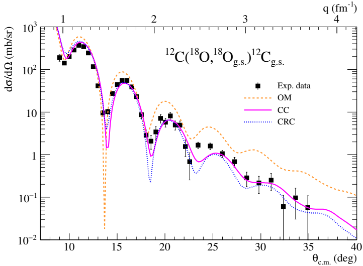
Figure 2. Experimental cross-section angular distribution of the ^{12}\text{C}(^{18}\text{O},^{18}\text{O}_{\text{g.s.}})^{12}\text{C}_{\text{g.s.}} elastic scattering at 275 MeV incident energy. Theoretical calculations for the elastic transition in OM, CC and CRC approaches are shown with the orange dashed, solid magenta and blue dotted lines, respectively.
