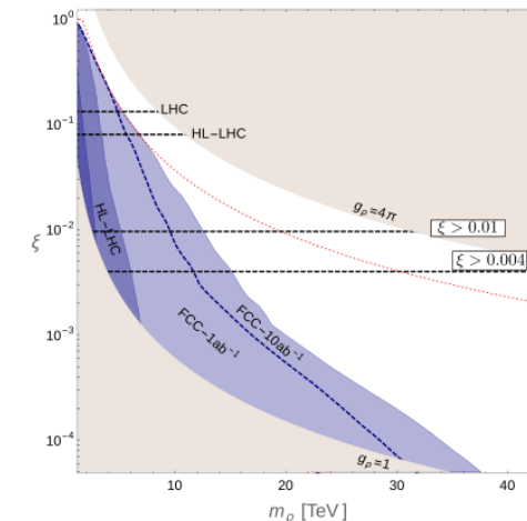
FCC CDR Vol. 1, Thamm, Torre, Wulzer, 1502.01701
