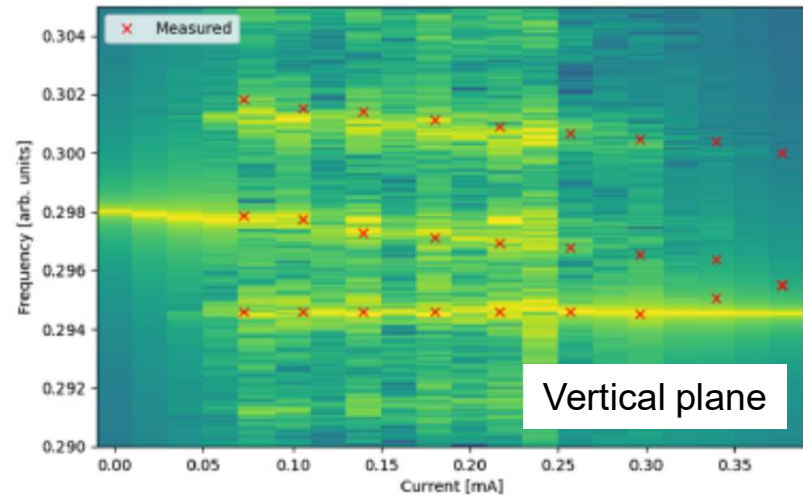
Mode shifts versus bunch current at chromaticity +1.5
