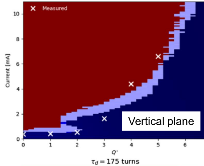
Instability thresholds as a function of chromaticity
