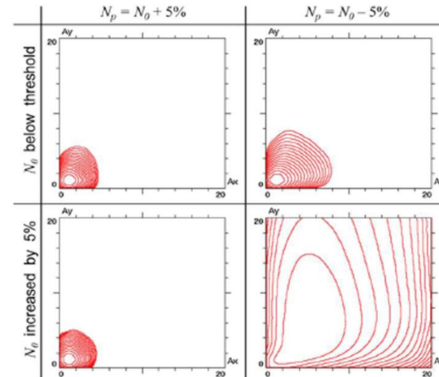
Density contour plots ( 1/e between successive lines) in the space of normalized betatron amplitudes.
