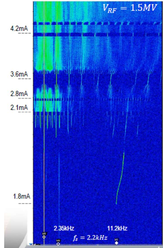
Beam spectra at 1.5 MV
