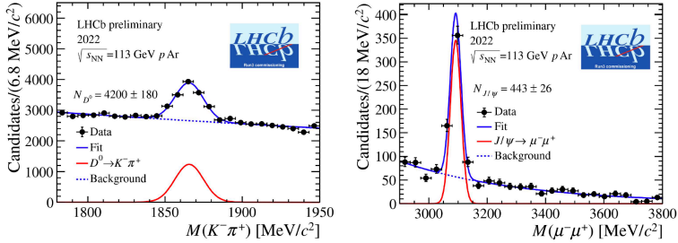
Figure 7. Early performance studies of the SMOG2 fixed-target system. These data were collected in 18 minutes of the LHC proton beam on fixed-target Ar collisions.
