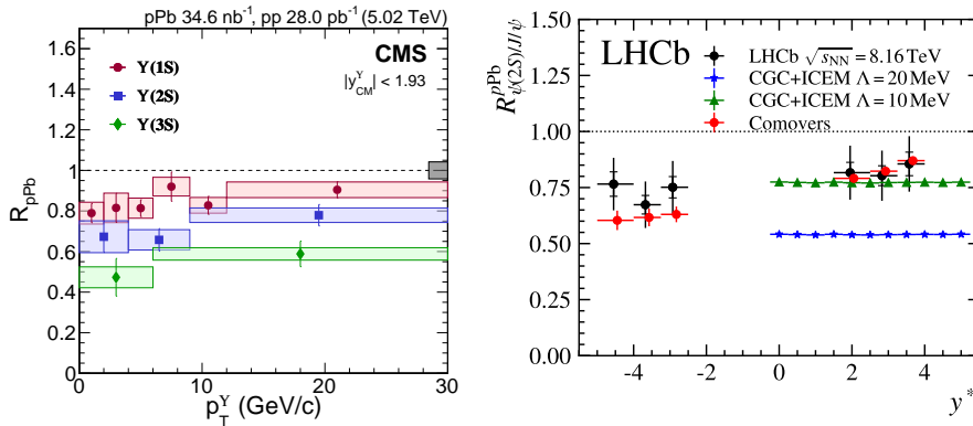
Figure 1. Left: R_{\text{pPb}} of \Upsilon(1S) (red), \Upsilon(2S) (blue) and \Upsilon(3S) (green) as functions of p_T obtained by the CMS experiment at 5.02 TeV [25]. Right: Double ratio of prompt \psi(2S) -to- J/\psi yields versus rapidity, measured in pPb at 8.16 TeV by the LHCb experiment [26] (black) and compared to glun saturation [27] (blue and green) and comover [13] (red) models.
