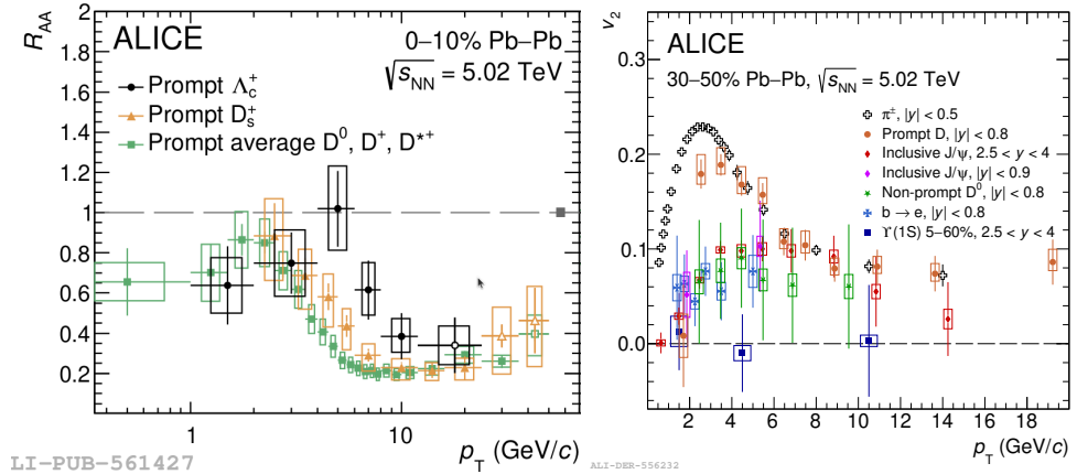
Figure 1. R_{AA} (left) for prompt \Lambda_c^+ baryon, D_s^+ meson, and average of D^0 , D^+ , D^{*+} mesons in 0–10% central Pb–Pb collisions and (right) elliptic-flow coefficient ( v_2 ) of various particle species in 30–50% central Pb–Pb collisions [9].
