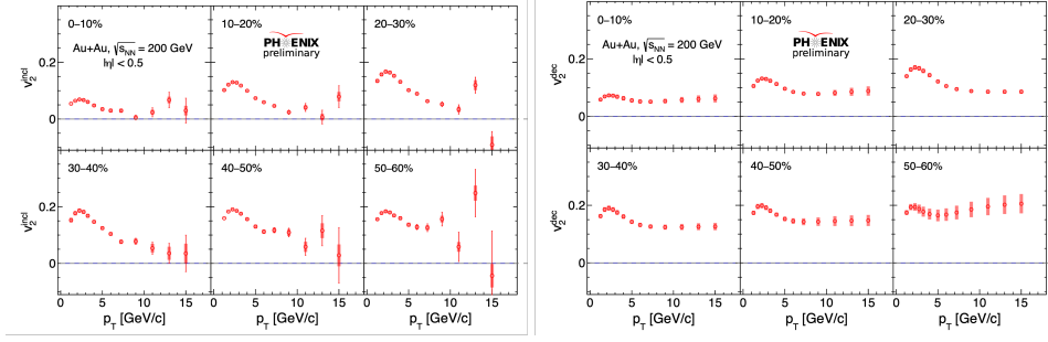
Figure 1. The v_2 for inclusive photons (left) and decay photons (right) measured in the PHENIX 2014 Au+Au dataset.
