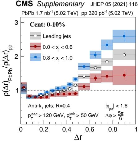
Figure 2. Ratios of PbPb to pp jet shapes for different x_j selections for leading (left) and subleading (right) jets. [4].
