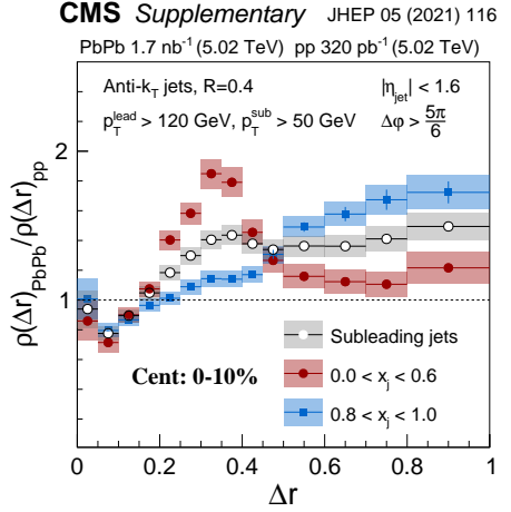
Figure 2. Ratios of PbPb to pp jet shapes for different x_j selections for leading (left) and subleading (right) jets. [4].
