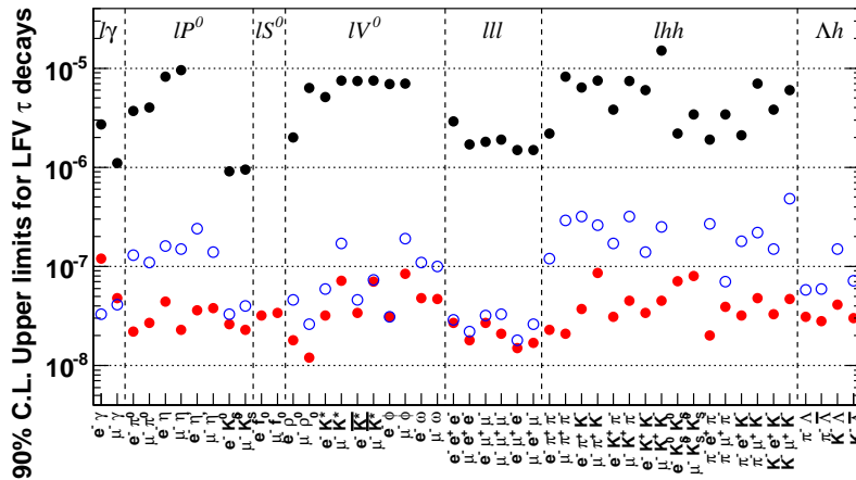
Figure 4. Current 90% CL ULs for the branching fraction of \tau LFV mode. Red, blue and black circles shows Belle, BaBar [6] and CLEO [7] results, respectively.
