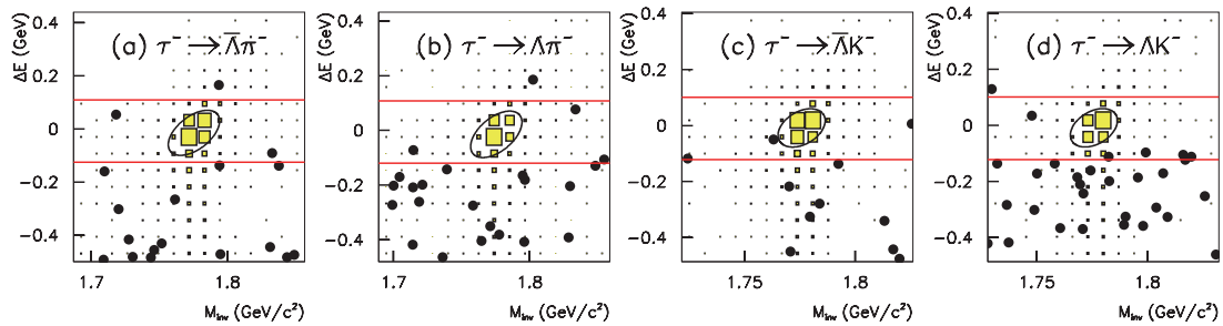
Figure 3. Resulting plots on the M_{\text{inv}} - \Delta E plane for \tau^- \rightarrow \bar{\Lambda} \pi^- (a), \tau^- \rightarrow \Lambda \pi^- (b), \tau^- \rightarrow \bar{\Lambda} K^- (c) and \tau^- \rightarrow \Lambda K^- (d). Here, black dots show the data and yellow boxes indicate the density for the signal events.
