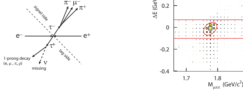
Figure 1. Left: Topology for the signal event, where the signal decay is \tau \rightarrow \mu\pi\pi . Right: Resulting distribution for the signal events on the M_{\text{inv}} - \Delta E plane. The size of boxes shows the magnitude of the density for the signal events, the red ellipse indicates the \pm 3\sigma signal region and the region between the two red lines is defined as the \pm 5\sigma_{\Delta E} side-band region for the background estimation.
