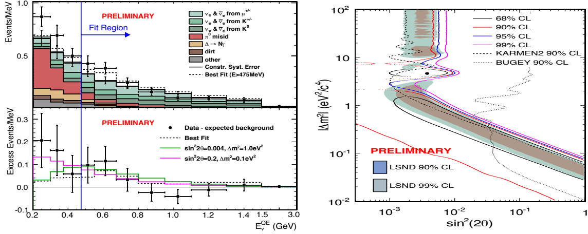
Figure 2. Top Left: Reconstructed E_{\nu} distribution of \bar{\nu}_e CCQE candidates in MiniBooNE anti-neutrino running. Bottom Left: The difference between the data and predicted backgrounds as a function of reconstructed neutrino energy. The error bars include both statistical and systematic components. Also shown in the figure are expectations from the best oscillation fit with E_{\nu} > 475 MeV, (\Delta m^2, \sin^2 2\theta) = (4.64 \text{ eV}^2, 0.00337) where the fit is extrapolated below 475 MeV and from other neutrino oscillation parameter sets in the LSND allowed region. Right: MiniBooNE 68%, 90%, and 99% C.L. allowed regions for events with E_{\nu} > 475 MeV within a two neutrino \bar{\nu}_{\mu} \rightarrow \bar{\nu}_e oscillation model. The black dot shows the best fit point.
