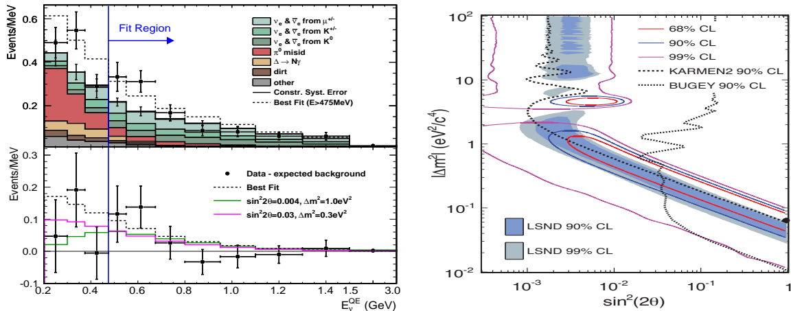
Figure 1. Results obtained with 5.66 \times 10^{20} POT exposure. Top Left: Reconstructed E_\nu distribution of \bar{\nu}_e CCQE candidates in MiniBooNE anti-neutrino running. Bottom Left: The difference between the data and predicted backgrounds as a function of reconstructed neutrino energy. The error bars include both statistical and systematic components. Also shown in the figure are expectations from the best oscillation fit with E_\nu > 475 MeV, (\Delta m^2, \sin^2 2\theta) = (0.064 \text{ eV}^2, 0.96) where the fit is extrapolated below 475 MeV and from other neutrino oscillation parameter sets in the LSND allowed region. Right: MiniBooNE 68%, 90%, and 99% C.L. allowed regions for events with E_\nu > 475 MeV within a two neutrino \bar{\nu}_\mu \rightarrow \bar{\nu}_e oscillation model, obtained with 5.66 \times 10^{20} POT exposure [6]. The shaded areas show the 90% and 99% C.L. LSND allowed regions. The black dot shows the best fit point.
