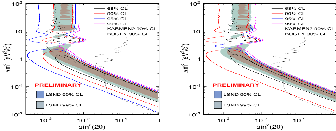
Figure 3. Left: MiniBooNE 90% and 99% C.L. allowed regions for events with E_\nu > 200 MeV within a two neutrino \bar{\nu}_\mu \rightarrow \bar{\nu}_e oscillation model. The shaded areas show the 90% and 99% C.L. LSND allowed regions. Right: MiniBooNE 90% and 99% C.L. allowed regions for events with E_\nu > 200 MeV within a two neutrino \bar{\nu}_\mu \rightarrow \bar{\nu}_e oscillation model, with the subtraction of the expected 17 event excess in the 200 < E_\nu < 475 MeV low-energy region from the neutrino component of the beam.
