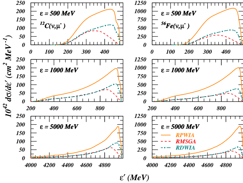
Figure 1. Cross sections for the charged-current reactions ^{12}\text{C}(\nu_\mu, \mu^-) and ^{56}\text{Fe}(\nu_\mu, \mu^-) as a function of the energy of the outgoing muon \varepsilon' . The different curves compare the RMSGA results (dashed) with the RDWIA (dash-dotted) and the RPWIA limit (full line).
