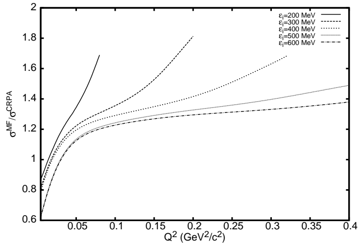
Figure 5. Ratio of cross sections obtained with mean field (MF) wave functions to cross sections including continuum RPA correlations (CRPA) as a function of Q^2 for incoming neutrino-energies ranging from 200 to 600 MeV and with ^{12}\text{C} as target nucleus.
