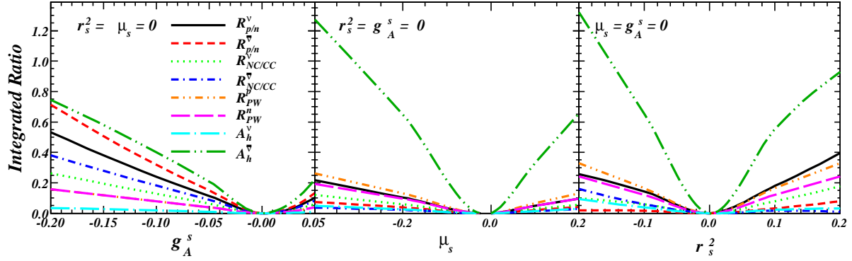
Figure 2. Comparison between the strangeness influence on various ratios of total cross-sections in terms of the relative sensitivity \left| \frac{R(s=0)-R(s)}{R(s=0)} \right| , as a function of the strangeness form factors g_A^s , \mu_s and r_s^2 for 1 GeV neutrino scattering off ^{12}\text{C} .
