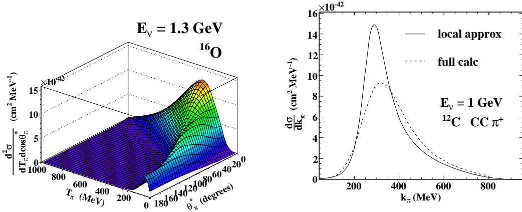
Figure 4. Comparison of full and local approximation calculations for coherent pion production.
