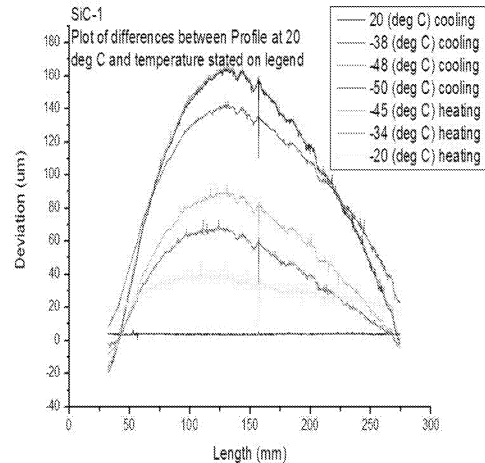
Fig. 6. Deviation from the original position as function of the location and temperature for the SiC ladder.
