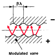
Modulated vane Adjacent vanes (90°)
