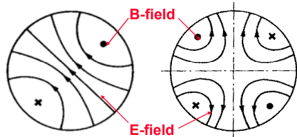
Empty cavity; mode TE 11 Empty cavity; mode TE 21
