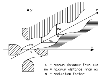
Modulated vane Adjacent vanes (90°)
