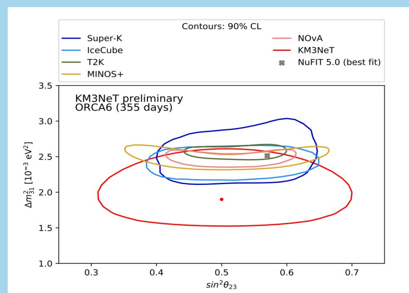
Fig.8 Contour at 90% CL of ORCA6 for the oscillation parameters \Delta m^2_{3,1} and \theta_{23} [4].
