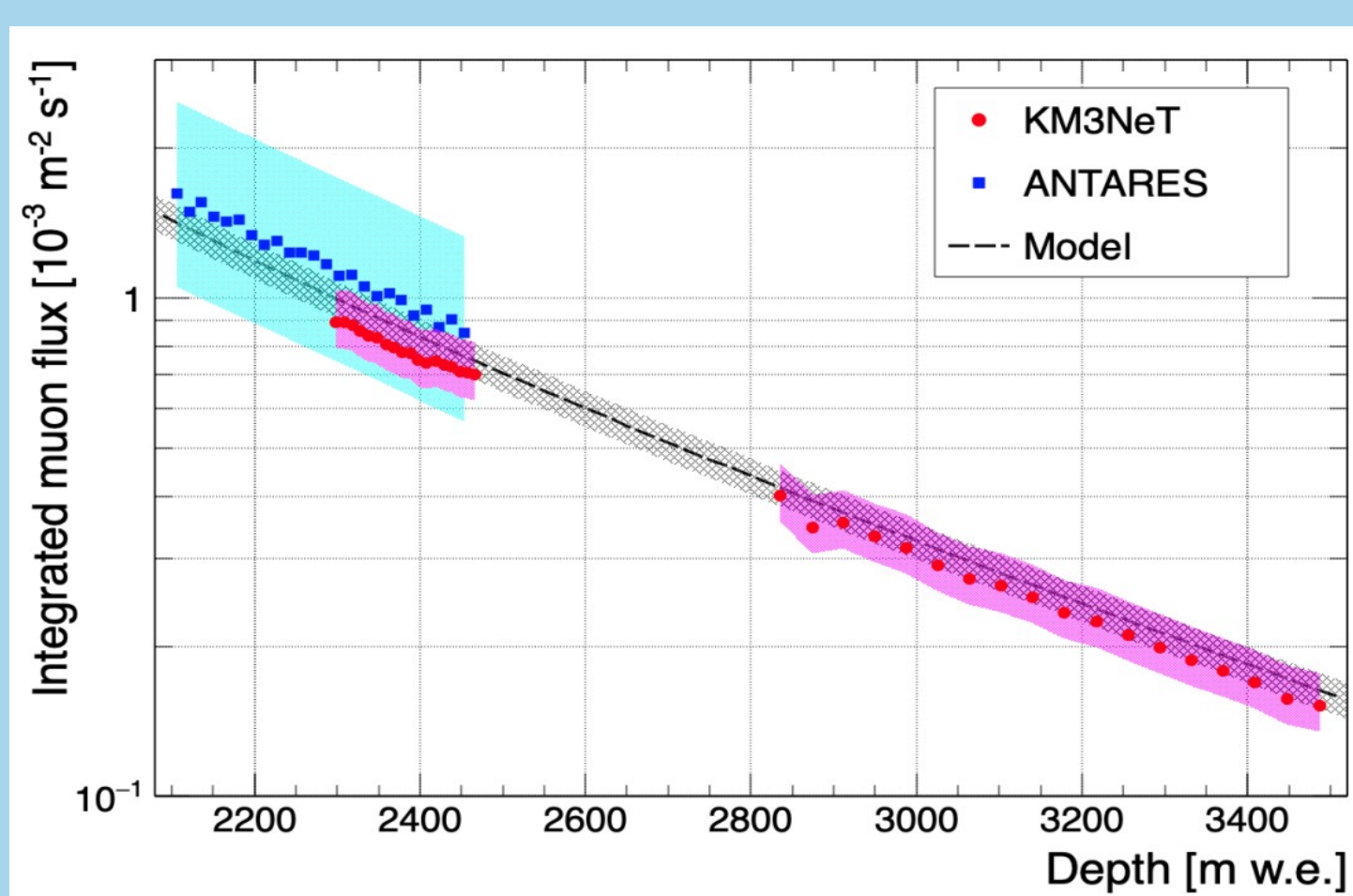
Fig.5 Integrated atmospheric muon flux measured with the ORCA1 and ARCA2 detectors as a function of depth below the sea level. The systematic errors are displayed as light red shadowed areas. The Bugaev model of the atmospheric muon flux is drawn with a dashed black line [2].
