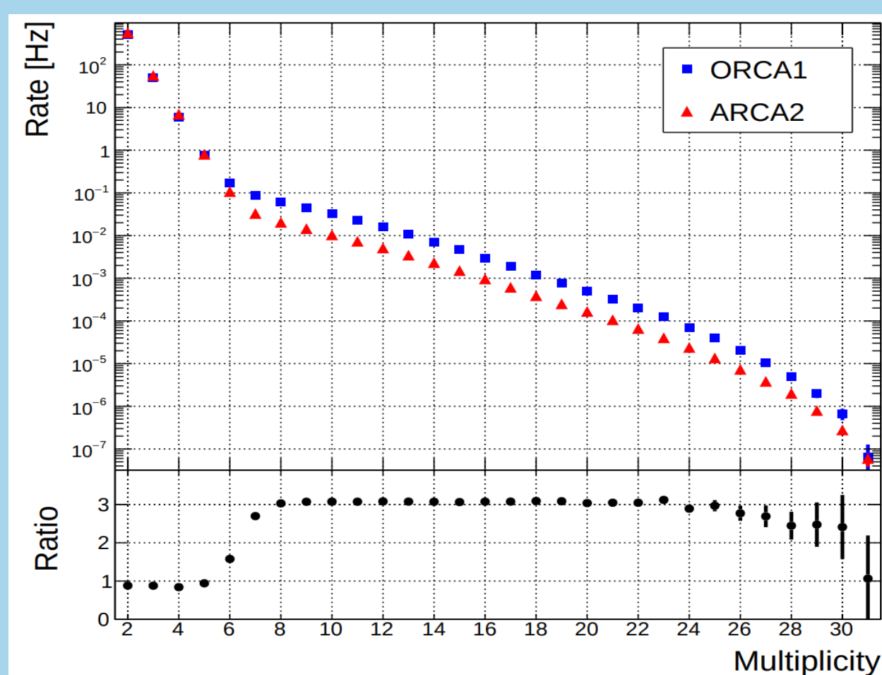
Fig.4 Coincidence rates as a function of the multiplicity for the ORCA1 and ARCA2 detectors averaged over all the DOMs of each detector [2].
