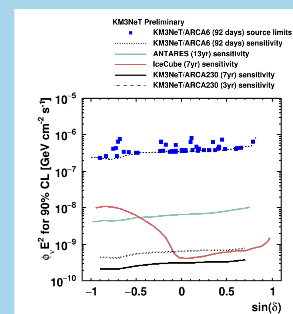
Fig.10 Limits and sensitivities of cosmic neutrino flux versus declination [5].
