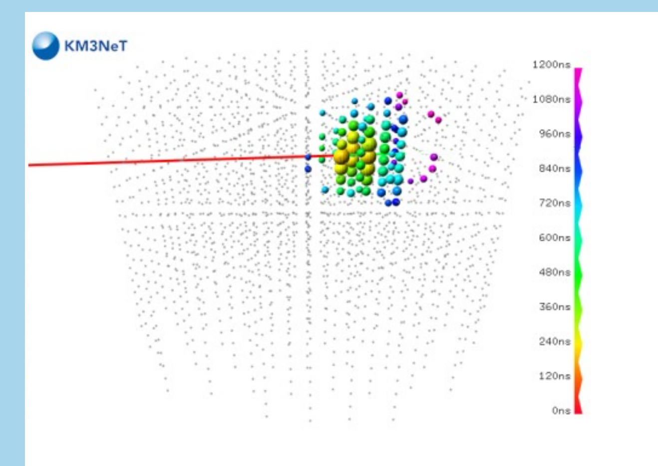
Fig.3 Shower-like event caused by the neutrinos interacting with seawater through neutral current interaction or charged current interaction of electron neutrino [1].
