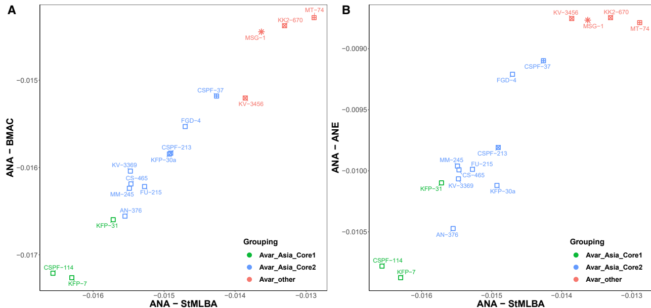
Figure 4. Two-dimensional f4-statistics of Avar_Asia_Core individuals
