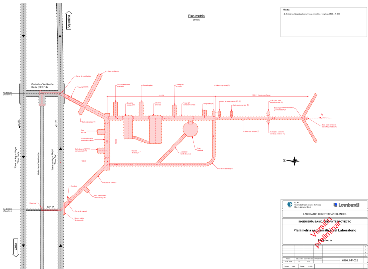
Figure 2: Final design for the ANDES deep underground laboratory, from the basic engineering phase [47]. See text for details.
