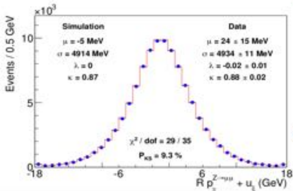
high p_T^Z
