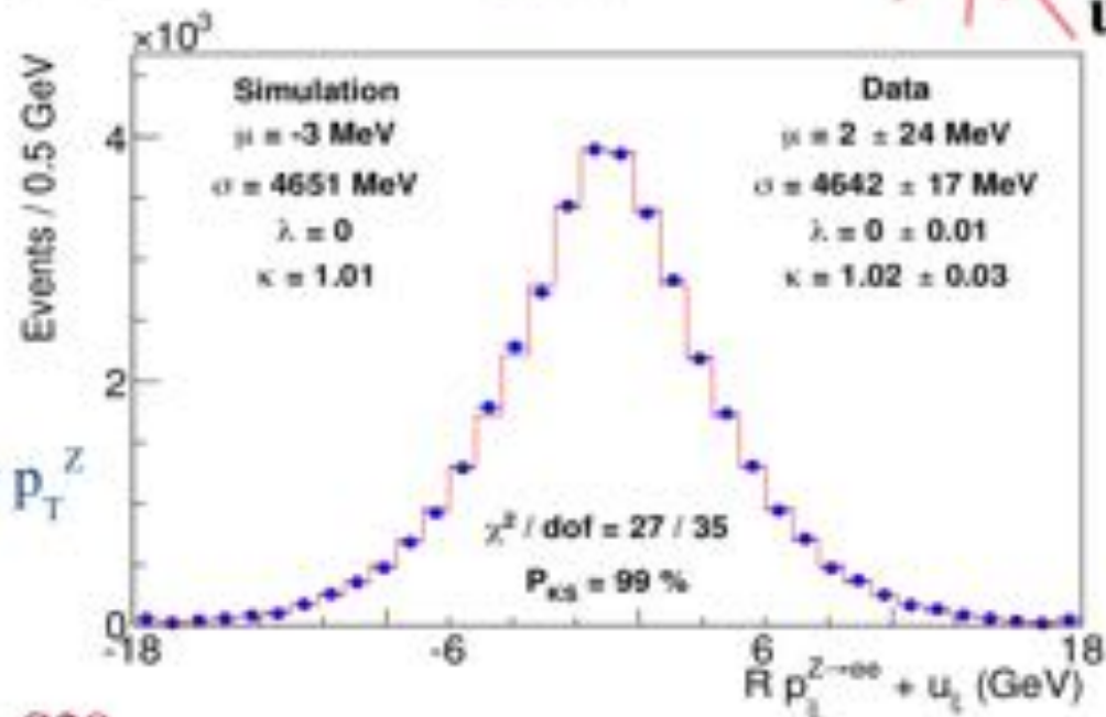
low p_T^Z
