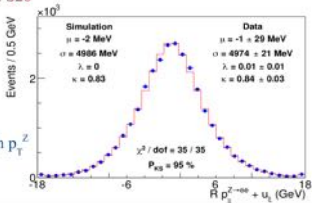
low p_T^Z
