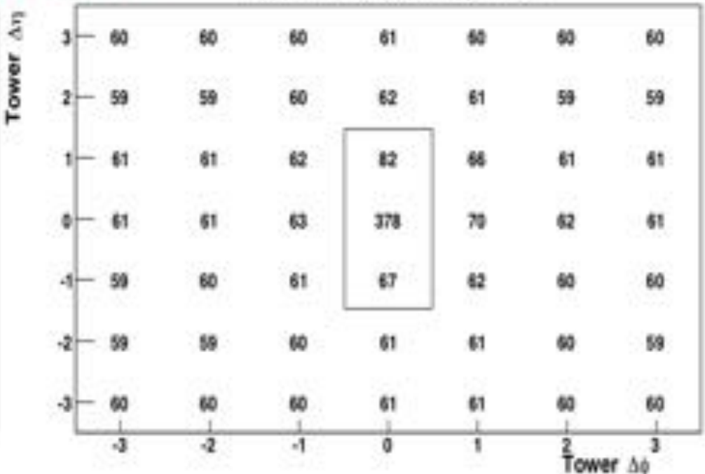
Muon Electromagnetic E_T (MeV)
