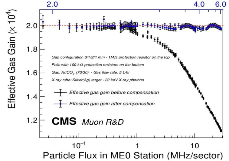
Nominal Operation Gain ( \times 10^4 )
