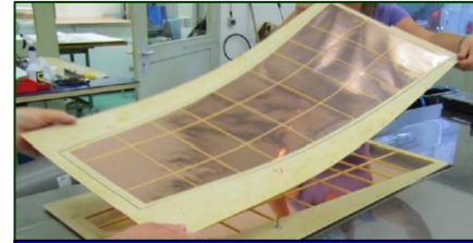
GEM foils on their frames
