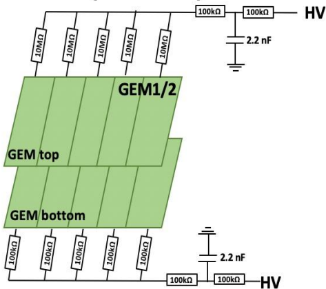
GE2/1 Baseline (validated)
