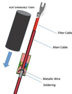
Filter application and connection to ground
