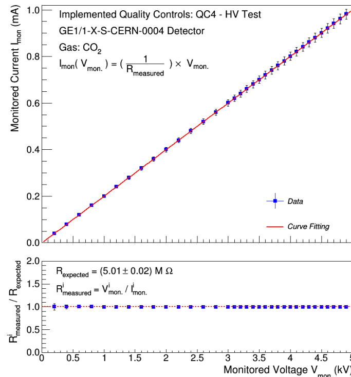
Typical I vs V curve obtained during the QC4 HV test. I mon. represents the current flowing through the HV divider to provide power to the detector electrodes.
