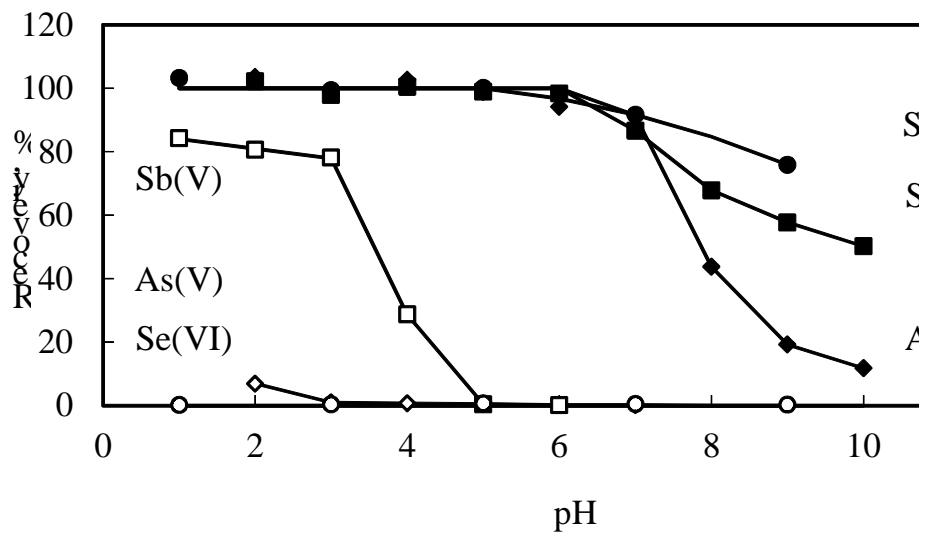
Fig. 2. Extraction Recoveries of Various Species by DBDC/MIBK at Different Aqueous pH
