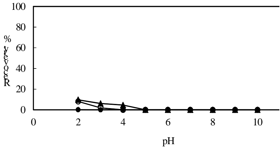
Fig. 3. Effect of pH on the Extraction of MMA, DMA and A by APDC/MIBK
