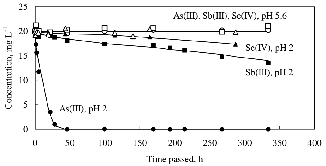
Fig. 6. Concentrations of As(III), Sb(III) and Se(IV) at Different Passed Time after been Extracted into MIBK
