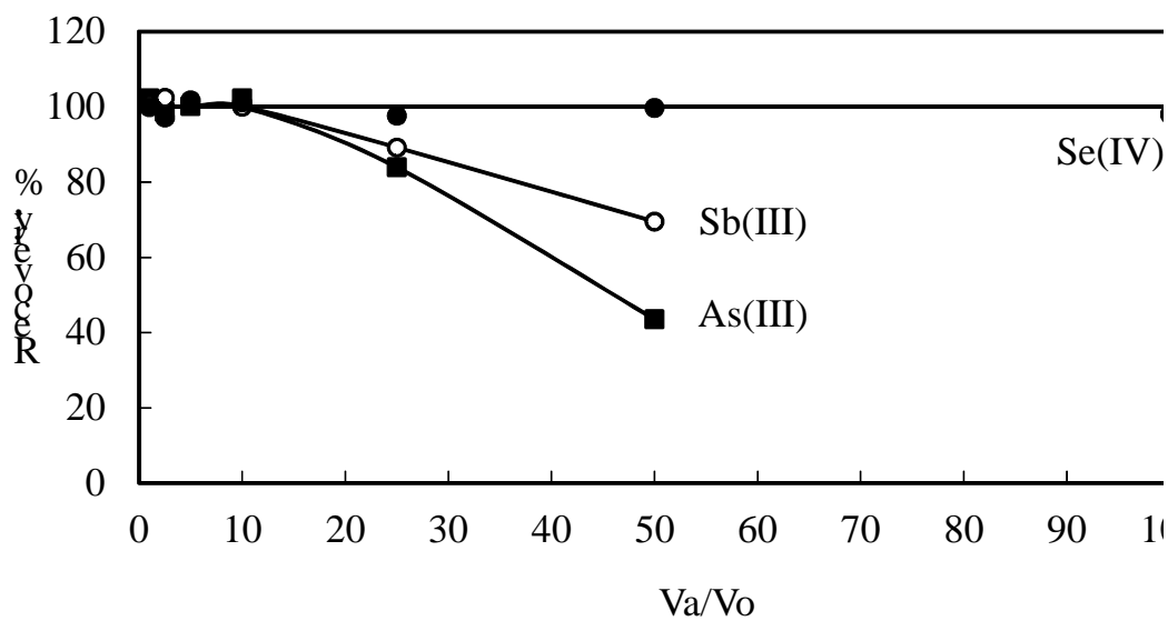
Fig. 4. Recoveries of As(III), Sb(III) and Se(IV) at Different Extraction Phase Volume Ratio
