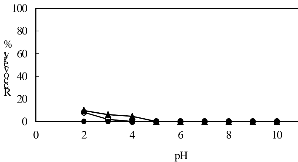
Fig. 3. Effect of pH on the Extraction of MMA, DMA and A by APDC/MIBK
