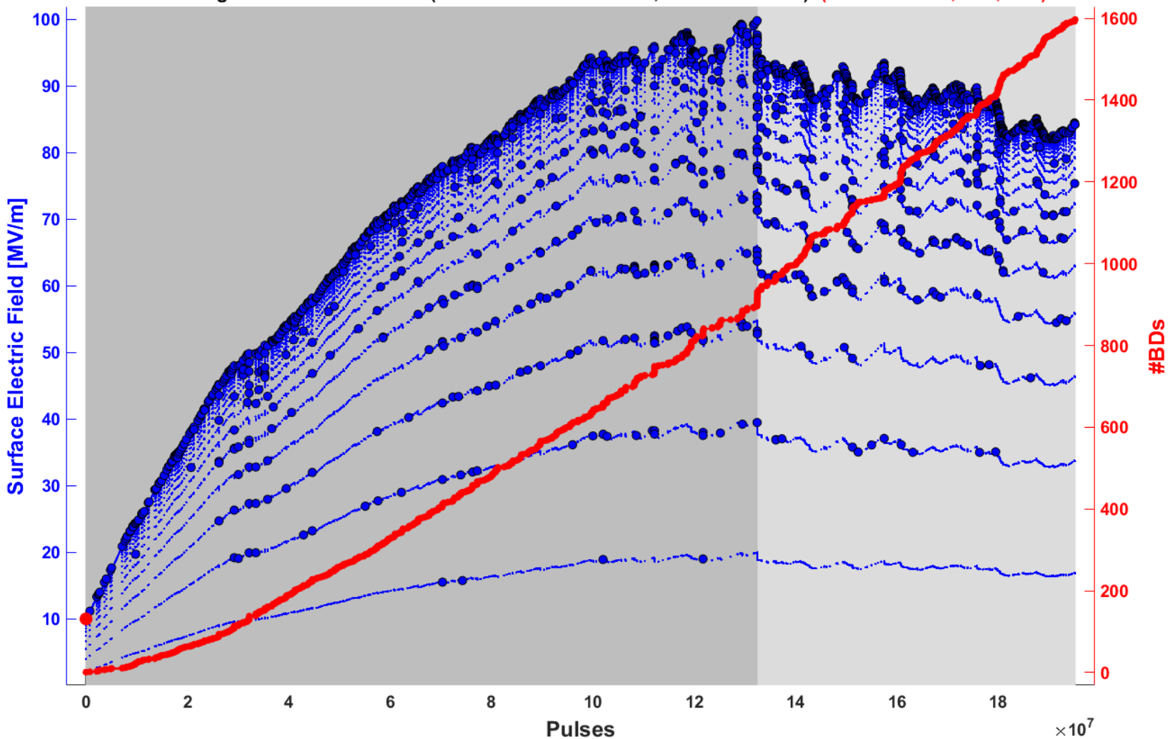
Conditioning curve for 024 Hard Cu (Total Pulses - 195204927, Total BDs - 1597) (T=3637901197, R=2, N=1)
