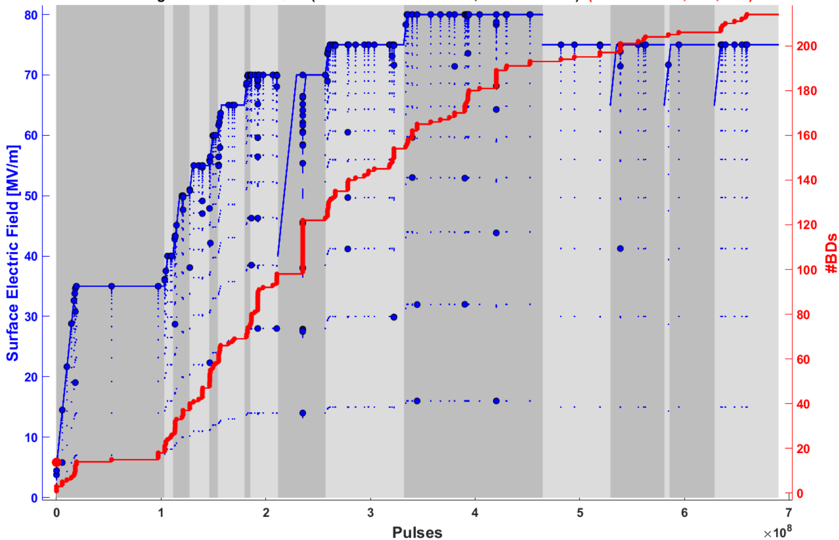
Conditioning curve for 045 RFQ Cu (Total Pulses - 689670047, Total BDs - 214) (T=3703564240, R=2, N=1)
