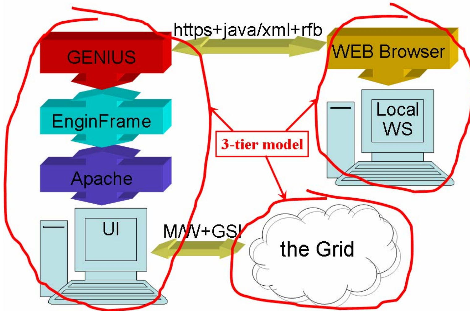
Three tier architecture of the GENIUS grid portal
