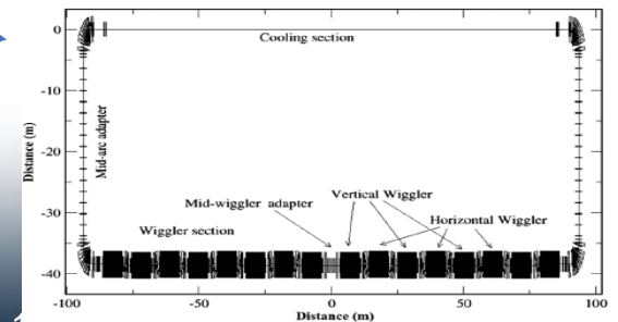
FIG. 2. Layout of the ring cooler.
