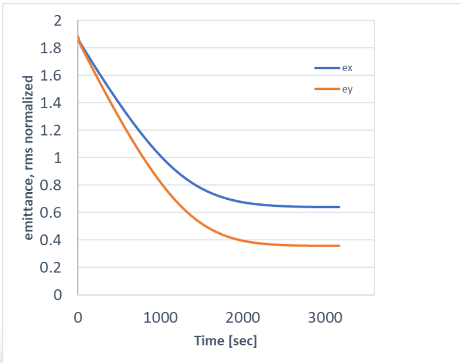
Fig. Cooling of protons at \gamma=25 , with decoupled transverse motion (IBS+Cooling only).
