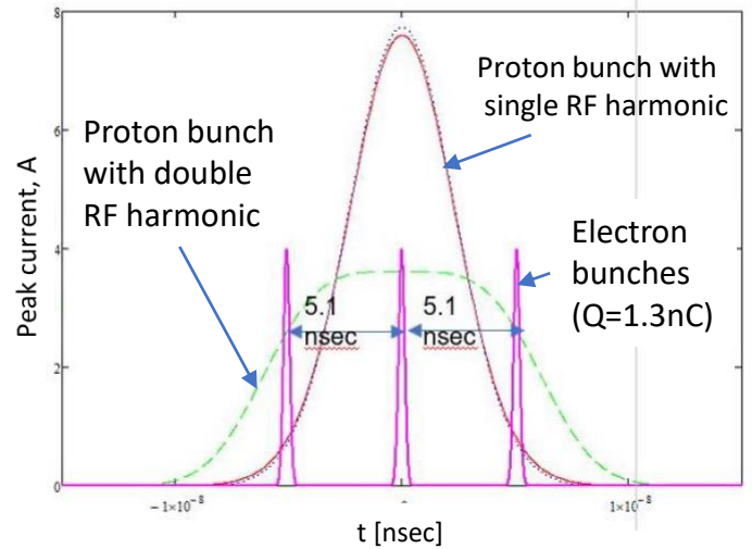
Fig. Electron beam time structure (3 electron bunches per single bunch of protons).
