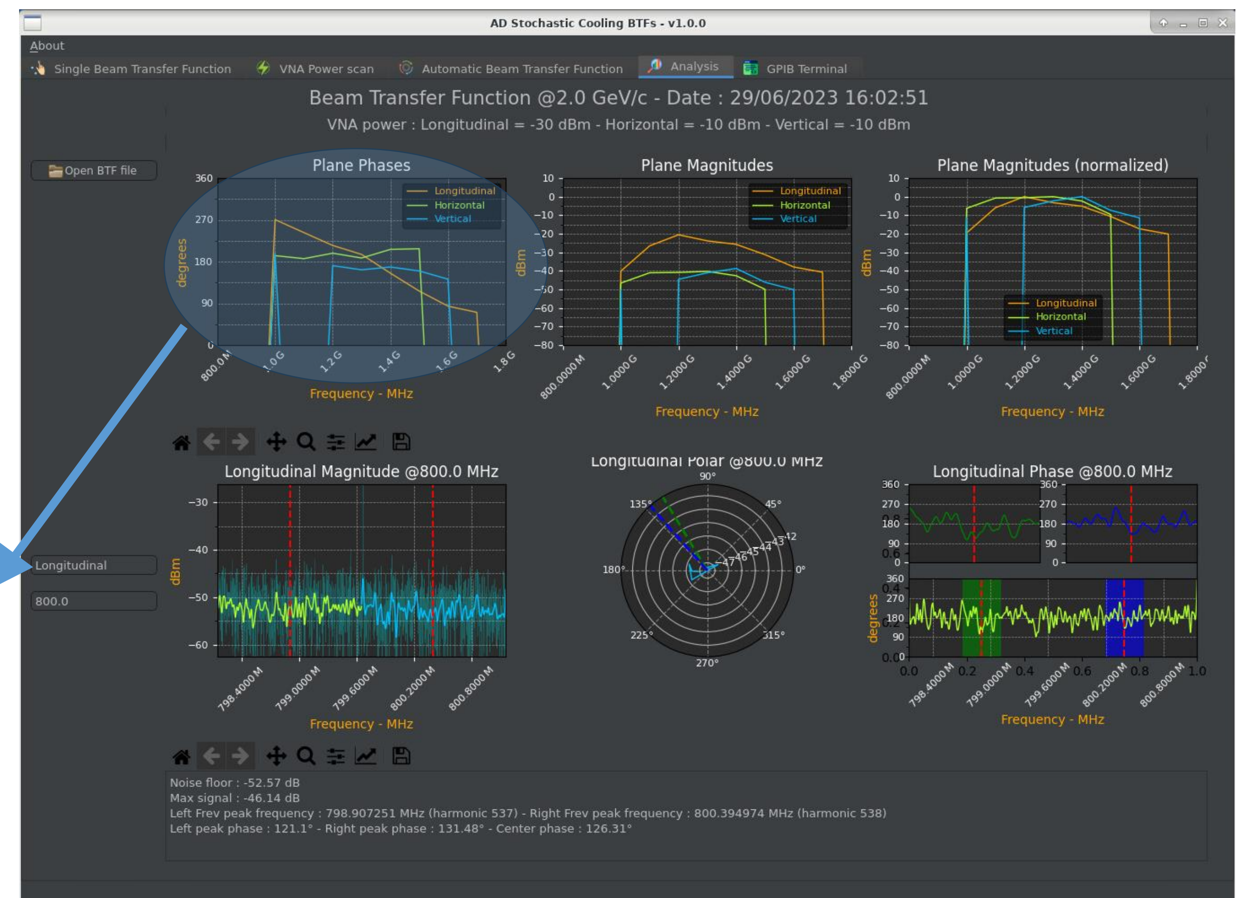
Figure 4 – Automated data analysis displaying measurement synthesis and enabling scrolling data
