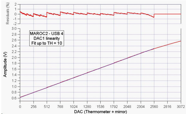
Figure 6: DAC linearity of the first discriminator.
