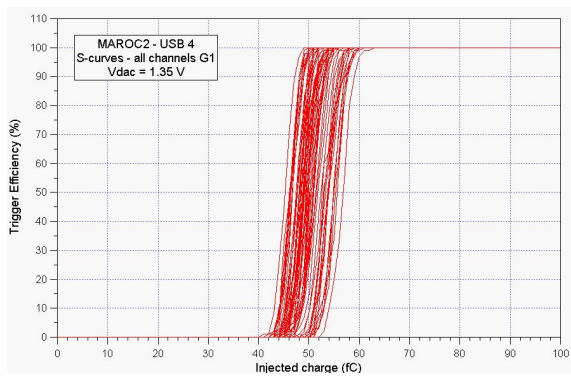
Figure 7: Trigger efficiency of the 64 channels of a chip as a function of the injected charge for a fixed threshold of 1.35 V, also called S-curves.
