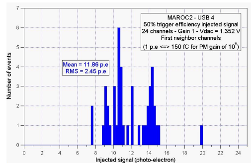
Figure 14: Injected signal for which cross-talk appears.
