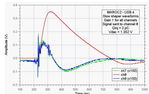
Figure 15: Slow shaper waveforms for channel 8 and its two neighbours for an injected charge of 2 pC on the central channel.
