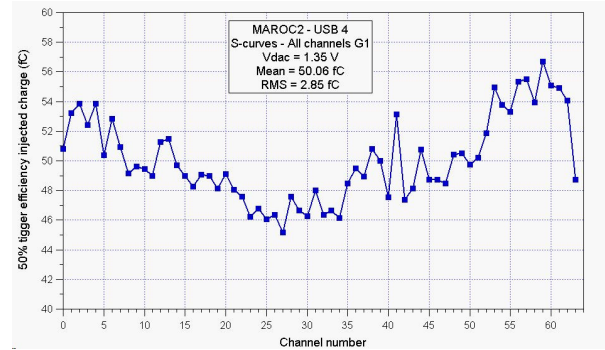
Figure 8: 50 % trigger efficiency input charge versus the channel number.
