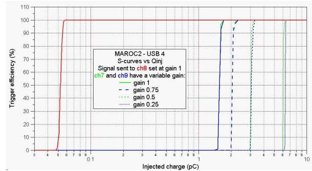
Figure 13: S-curves for channel 9 at gain 1 and its two neighbours for four different gains in the range [0.25, 1].
