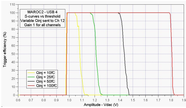
Figure 11: Trigger efficiency as a function of the threshold applied for 4 different injected charges.
