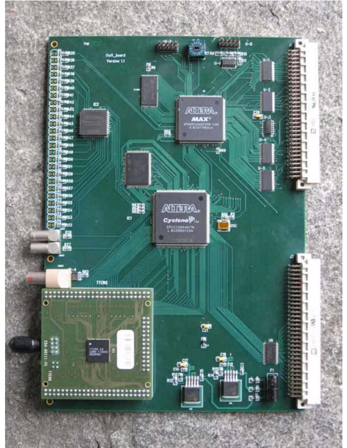
Figure 5: TTCit board
