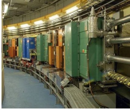
PS_Booster: 1.4 GeV
