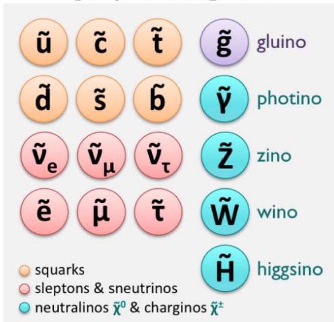
Supersymmetric partners
