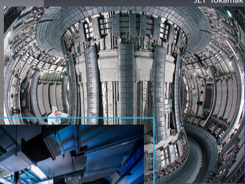
JET Tokamak
