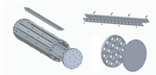
Figure 4: Computerized sketch of where the magnets will be coupled.
