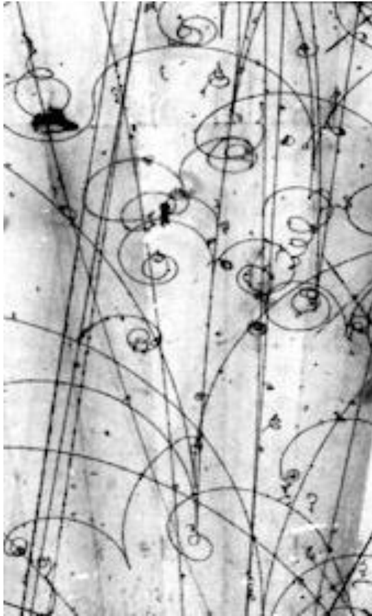
Fermilab: Bubble Chamber Photo
