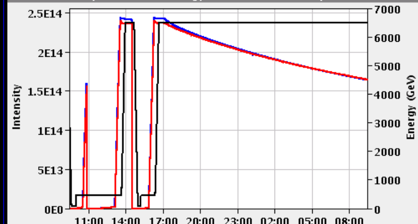
FBCT Intensity and Beam Energy Updated: 09:25:43
