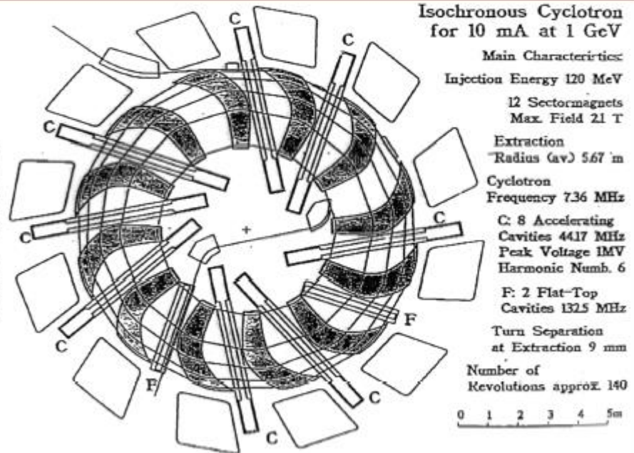
Fig. 4. Layout of the proposed high power cyclotron.
