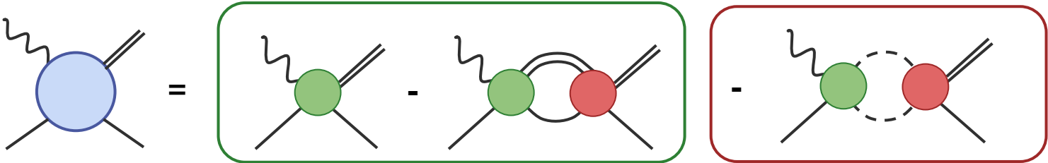
Indirect contributions from coupled channels
