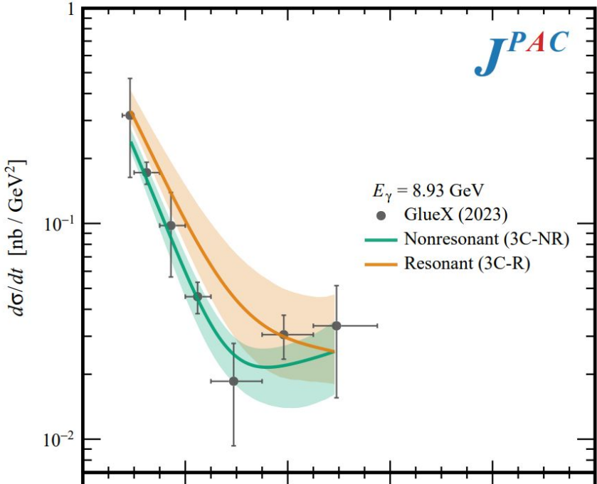
All reproduce apparent enhancement at large |t| !
