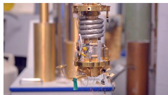
Device to study quantum turbulence in superfluid ^4\text{He} .
