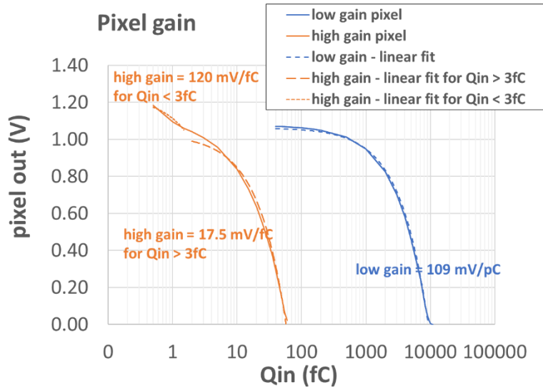
Fig. 2. Gain as a function of Q_{in} for both pixel designs.
