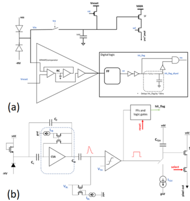
Fig. 1. (a) Low gain pixel architecture. (b) High gain pixel architecture.
