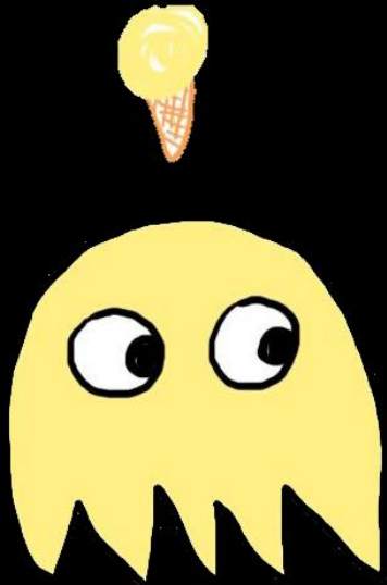
electron neutrino
