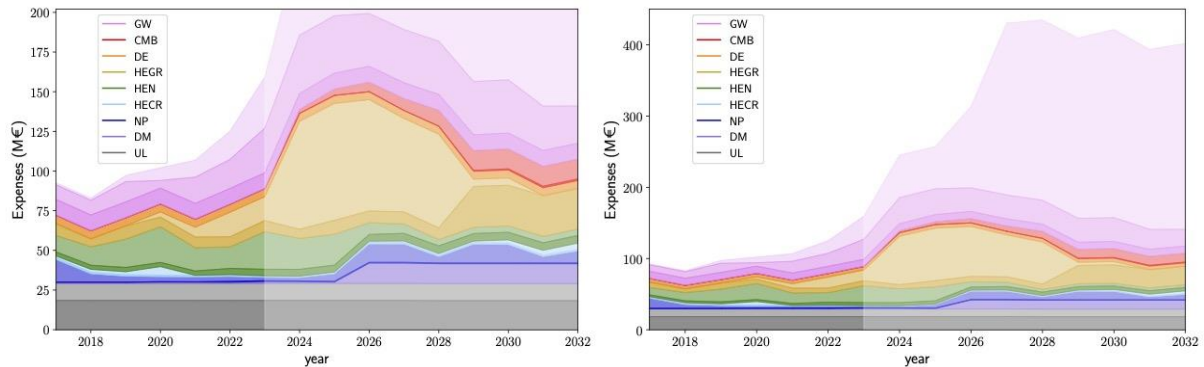
Figure 1: Estimate of realised and planned investment and exploitation expenditures in Astroparticle Physics. The division of the APP sub-fields is UL: underground laboratories; DM: Dark Matter experiments; NP: Neutrino Properties experiments; HEGR: High-Energy Gamma Ray observatories and satellite missions; HEN: High-Energy Neutrino observatories; HEGR: High-Energy Gamma Ray observatories and satellite missions; DE: Dark-Energy observatories and satellite missions; CMB: Cosmic Microwave Background observatories and satellite missions; GW: Gravitational Wave observatories and satellite missions. The exploitation is given by the darker shade for each colour and the investment budget by the lighter shade. For Gravitation Waves, three shadings have been used: dark for exploitation, middle tone for investments (to be) covered by the usual funding agencies and light for investments from exceptional sources, such as national, regional or EU (economic) structure funds. The part after 2023 has increasing uncertainties on the difference between planned and realised expenditures as time goes on. The left-hand side figure has a truncated vertical scale to make the relative magnitudes of the sub-fields apart from Gravitation Waves better visible.
