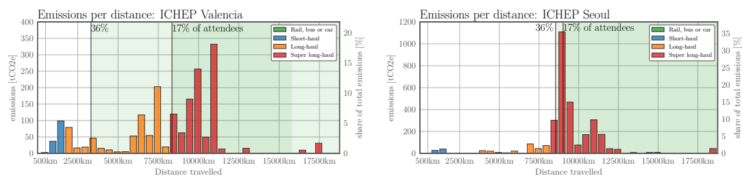
Figure 7.2: Emissions per distance for the different ICHEP editions shown in tCO 2e (left axis) and as share of the total emissions. Additionally, the emissions caused by the 17 % and 36 % participants furthest away are shaded in green.
