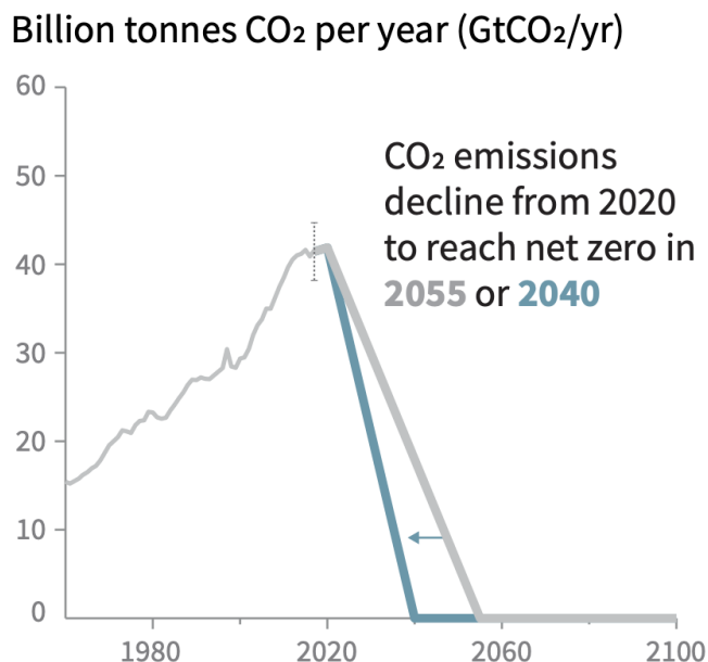
Figure 1.1: According to IPCC, the global net CO 2 emissions have to come down to zero to limit global warming and to avoid irreversible tipping points. A reduction until 2055 will have a probability of only 66 % to limit the temperature rise to 1.5°C (grey stylised pathway). Therefore, IPCC proposes to reach net-zero already in 2040 as shown in the blue stylised pathway to have a higher chance of limiting warming to 1.5°C. Figure from Ref. [5].
