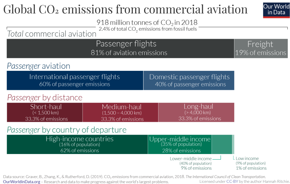
Figure 7.1: Global CO 2 emissions from commercial aviation, reproduced from Our World in Data [140], based on data from Ref. [141].
