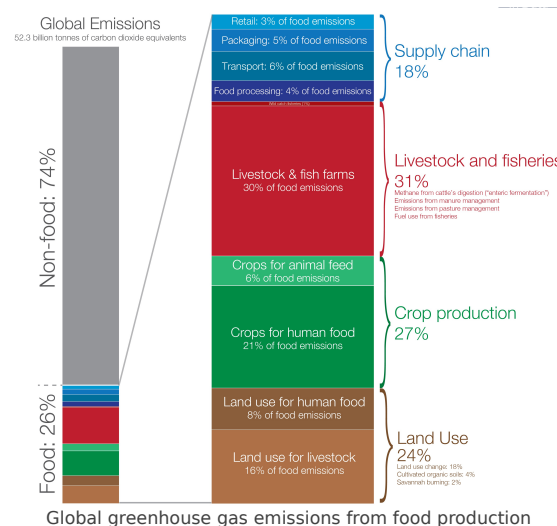
Figure 4.1: The graph shows the GHG emissions from the food sector and categorises it into emissions from livestock and fisheries, crop production (used directly for human consumption and used as livestock feed), land use, and the supply chain. Figure reproduced from Ref. [81], based on data from Ref. [82].
