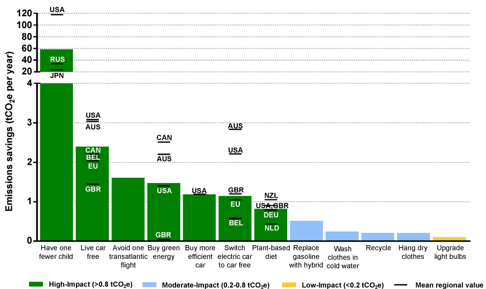
Figure 1.4: Emissions reduction from individual actions. Black lines correspond to individual developed nations studied, the mean over which is shown as a coloured bar. Note that these numbers are based on average current emissions in developed countries, and neglecting the effects of climate policy. The break in the left-most bar distinguishes between the emissions due to direct offspring and integrated emissions over all generations of descendents. Moreover the integrated estimate assumes emissions per capita that are constant in time. See the accompanying text for a more detailed exposition of the underlying assumptions and leading systematic uncertainties. Figure taken from Ref. [14]
