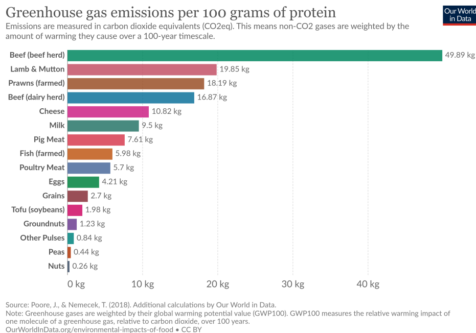
Figure 4.3: Greenhouse gas emissions in CO 2 e per 100 g of protein. Figure reproduced from Ref. [81], based on data from [82].
