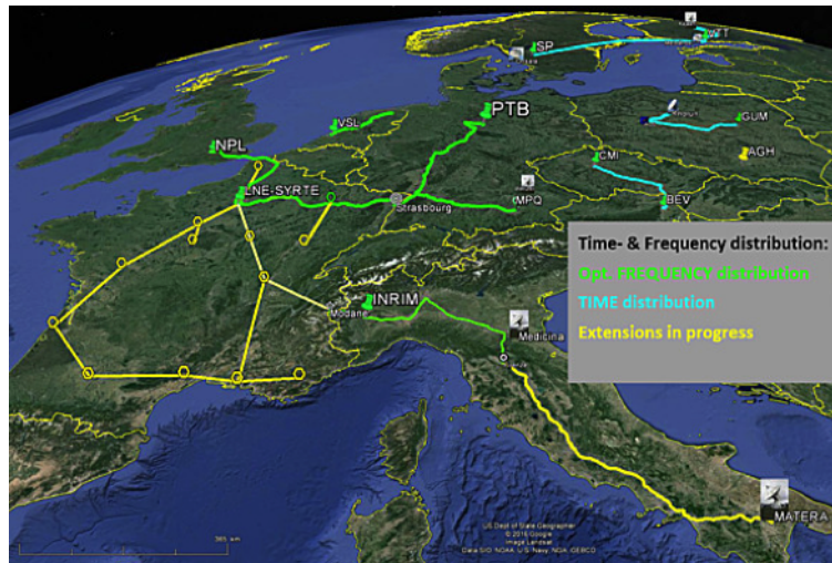
Figure 1: Existing and future trans-national optical clock network
