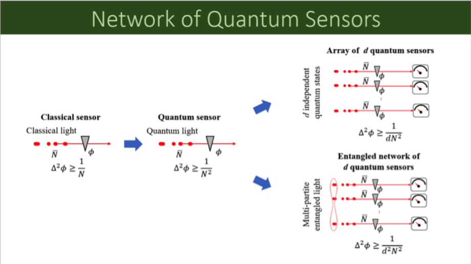
Figure 2: The improvement in sensitivity that entanglement can bring to a set of individual nodes of quantum sensors scales with the number of nodes.
