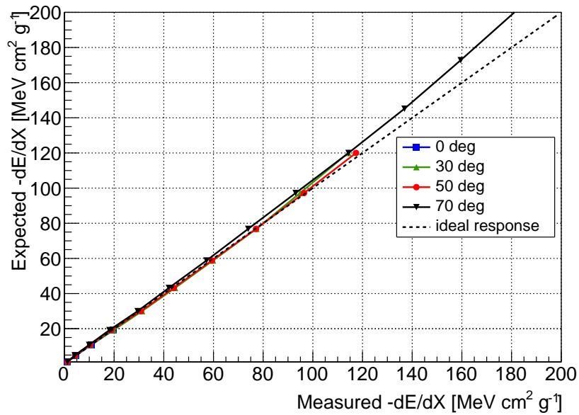
Figure 2: Comparison of measured and expected dEdX for the measurements in the mixed ion beam at different angles. The expected energy losses for ions are calculated following the Bethe-Bloch equation.
