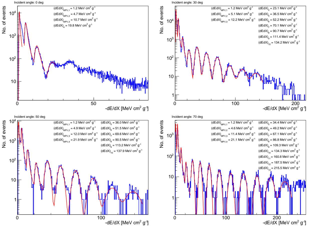
Figure 1: Comparison of the dE/dX measured in a mixed ion beam for the different impact angles investigated. Using spectrum stripping by iterative Landau- and Gaus-curve fitting different ion species are identified.
