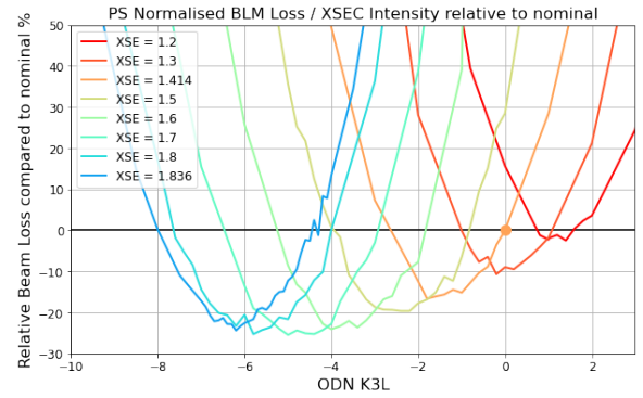
Figure 5: Measurements of relative beam loss reduction (y-axis) with octupole strength (x-axis) and sextupole strength (colour gradient), compared to nominal settings (orange dot).
