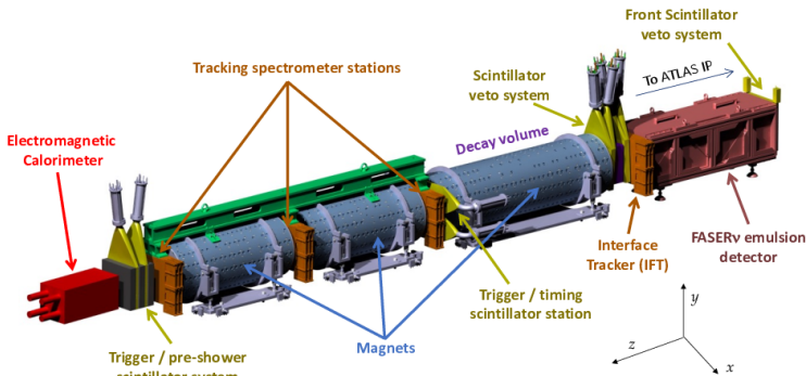
Figure 3. A schematic view of the FASER detector [13].
