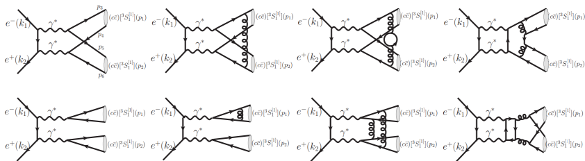
Figure 1. Several representative Feynman diagrams for e^+e^- \rightarrow (c\bar{c})[{}^3S_1^{[1]}] + (c\bar{c})[{}^3S_1^{[1]}] . 23 / 31
