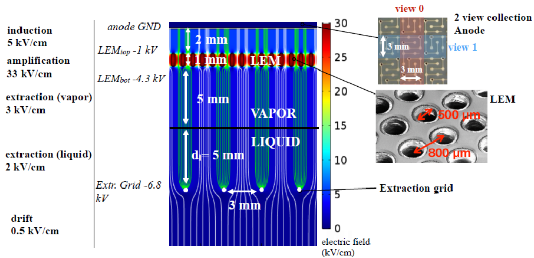
Figure 4.3. Thicknesses and [HV] values for electron extraction from liquid to gaseous argon, their multiplication by [LEMS] and their collection on the x and y readout anode plane. The [HV] values are indicated for a drift field of 0.5 kV/cm in [LAR] .
