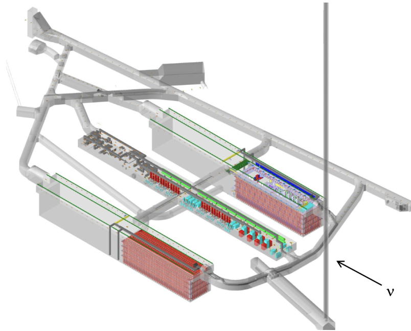
Figure 1.4. Underground caverns for the DUNE FD and cryogenics systems at SURF in South Dakota. The drawing shows the cryostats (red) for the first two FD modules in place at the 4850L . The Ross Shaft, the vertical shaft that will provide access to the DUNE underground area, appears on the right. Each cryostat is 65.8 m long (216 ft, approximately the length of two and a half tennis courts), 18.9 m wide, and 17.8 m tall (about three times as tall as an adult giraffe). The two detector caverns are each 144.5 m long, 19.8 m wide, and 28.0 m high, providing some room around the cryostats.
