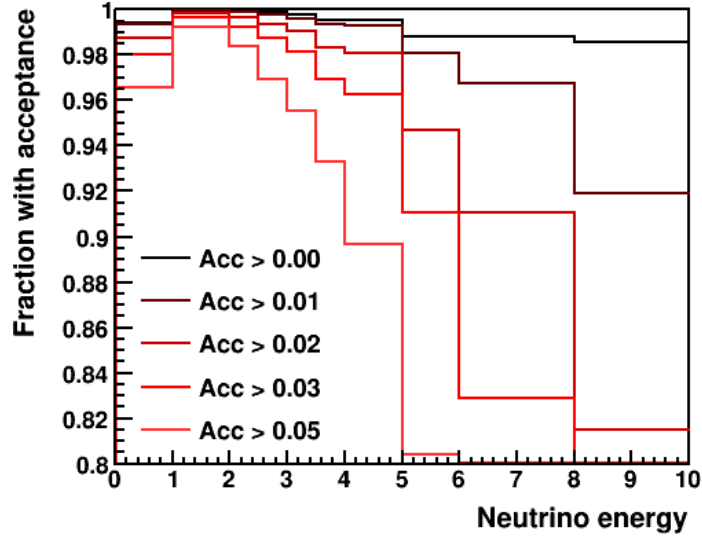
Figure A.12. This figure summarizes the neutrino acceptance in the (q_3, q_0) plane, as shown in figure A.11 , for all bins of neutrino energy (plotted in GeV). Here the quantity on the vertical axis is the fraction of events that come from bins in (q_3, q_0) with an acceptance greater than A_{cc} . As an example we consider the 4.0-5.0 GeV neutrino energy bin. The A_{cc} > 0.03 curve in that neutrino energy bin indicates that 96% of events come from (q_3, q_0) bins that have an acceptance greater than 3%.
