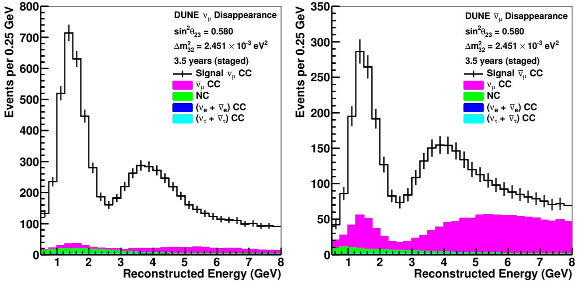
Figure 2.5. \nu_\mu and \bar{\nu}_\mu disappearance spectra: reconstructed energy distribution of selected \nu_\mu \overline{\text{CC}} -like events assuming 3.5 years (staged) running in the neutrino-beam mode (left) and antineutrino-beam mode (right), for a total of seven years (staged) exposure. The plots assume normal mass ordering.
