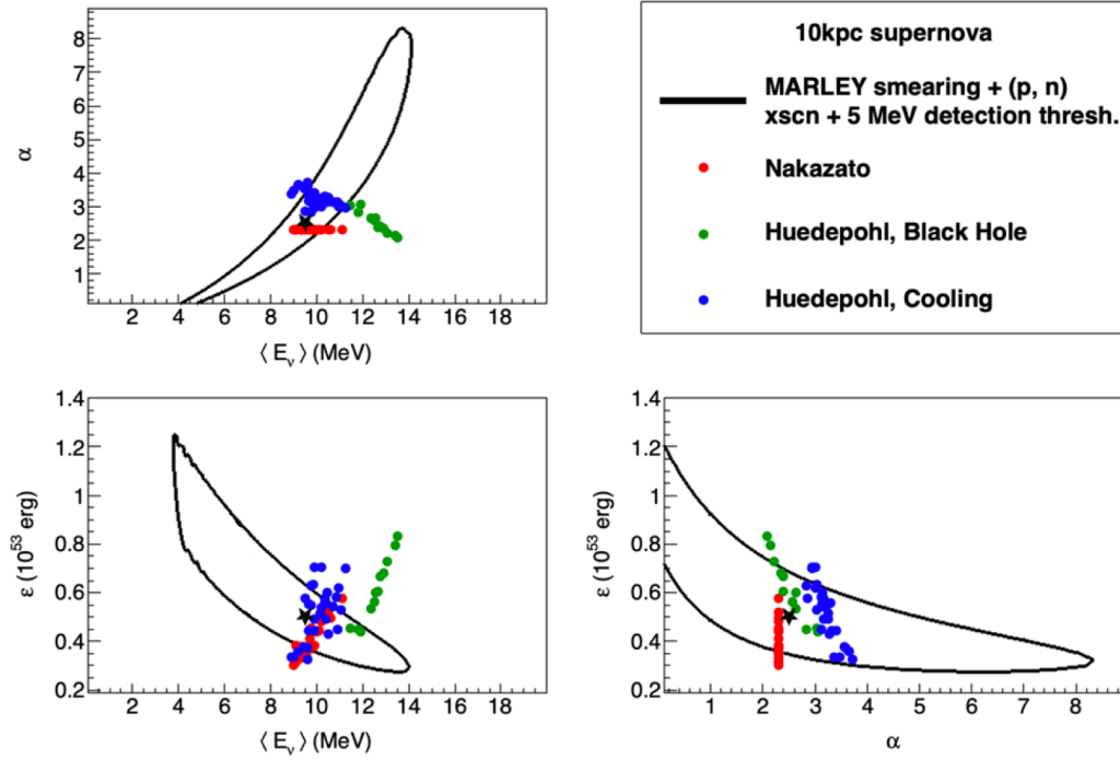
Figure 2.14. Estimated sensitivity regions for DUNE 's determination of the three supernova spectra parameters at 90% C.L. given the assumed true value indicated by the black star. The simulated data were generated for a supernova at 10 kpc with a neutrino interaction model appropriate for low energies, realistic detector smearing, and a step efficiency function with a 5 MeV detected energy threshold. To indicate the expected range of possible true flux parameters, superimposed are parameters corresponding to the time-integrated flux for three different sets of models: Nakazato [32], Huedepohl black hole formation models, and Huedepohl cooling models [33]. For the Nakazato parameters (for which there is no explicit pinching, corresponding to \alpha = 2.3 ), the parameters are taken directly from the reference; for the Huedepohl models, they are fit to a time-integrated flux.
