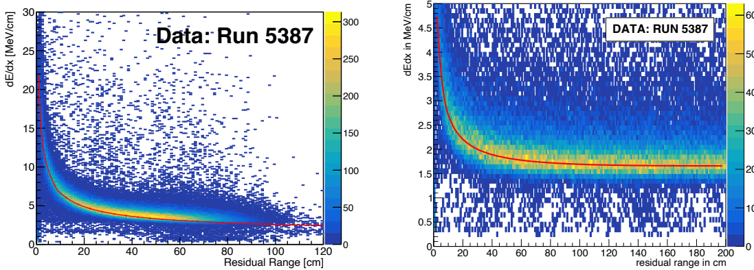
Figure 2.13. Energy loss of protons (left) and muons (right) in 1-GeV running with the ProtoDUNE-SP LArTPC at CERN , as a function of residual range. The protons are beam particles identified from beamline instrumentation; the muons are reconstructed stopping cosmic rays collected concurrently. The red curves represent the mean of the corresponding expected signature. Note the difference in the vertical scale of the two plots. The kaon dE/dx curve will lie between the two curves shown.
