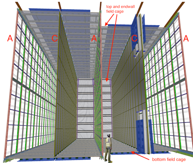
Figure 1.7. A 10 kt DUNE FD SP module , showing the alternating 58.2 m long (into the page), 12.0 m high anode (A) and cathode (C) planes, as well as the field cage (FC) that surrounds the drift regions between the anode and cathode planes. On the right-hand cathode plane, the foremost portion of the FC is shown in its undeployed (folded) state.
