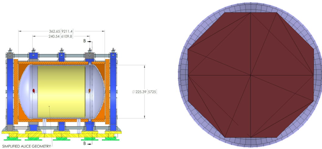
Figure A.22. On the left, the conceptual design of the MPD system for the ND . The ECAL (orange) is located outside the HPgTPC pressure vessel. On the right, a conceptual design of the ECAL endcap system.
