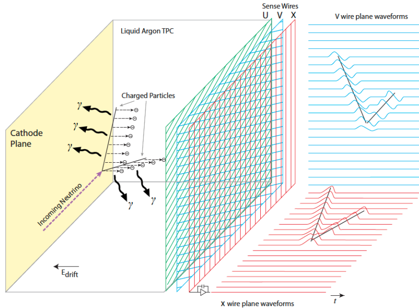
Figure 1.5. The general operating principle of the SP LArTPC . Negatively charged ionization electrons from the neutrino interaction drift horizontally opposite to the E field in the LAr and are collected on the anode, which is made up of the U, V and X sense wires. The right-hand side represents the time projections in two dimensions as the event occurs. Light ( \gamma ) detectors (not shown) will provide the t_0 of the interaction.
