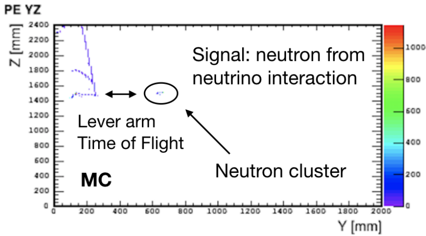
Figure A.44. An example of the antineutrino interaction in a 2.4 \times 2.4 \times 2.0 \text{ m}^3 3DST . The number of photoelectrons (PE) is plotted. An isolated cluster of hits corresponds to a neutron indirect signature produced by the antineutrino interaction.
