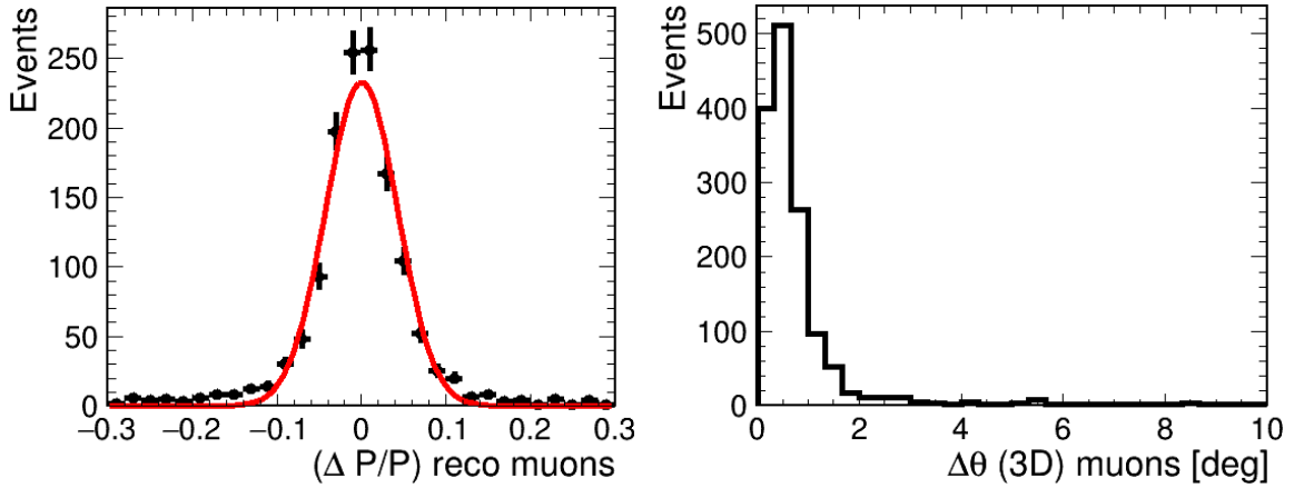
Figure A.31. Left: the momentum resolution for reconstructed muons in GArSoft, in a sample of 2 GeV \nu_\mu [CC] events simulated with [GENIE]. The Gaussian fit to the \Delta p/p distribution has a width of 4.2%. Right: the 3D angular resolution for the same sample of muons in GArSoft.
