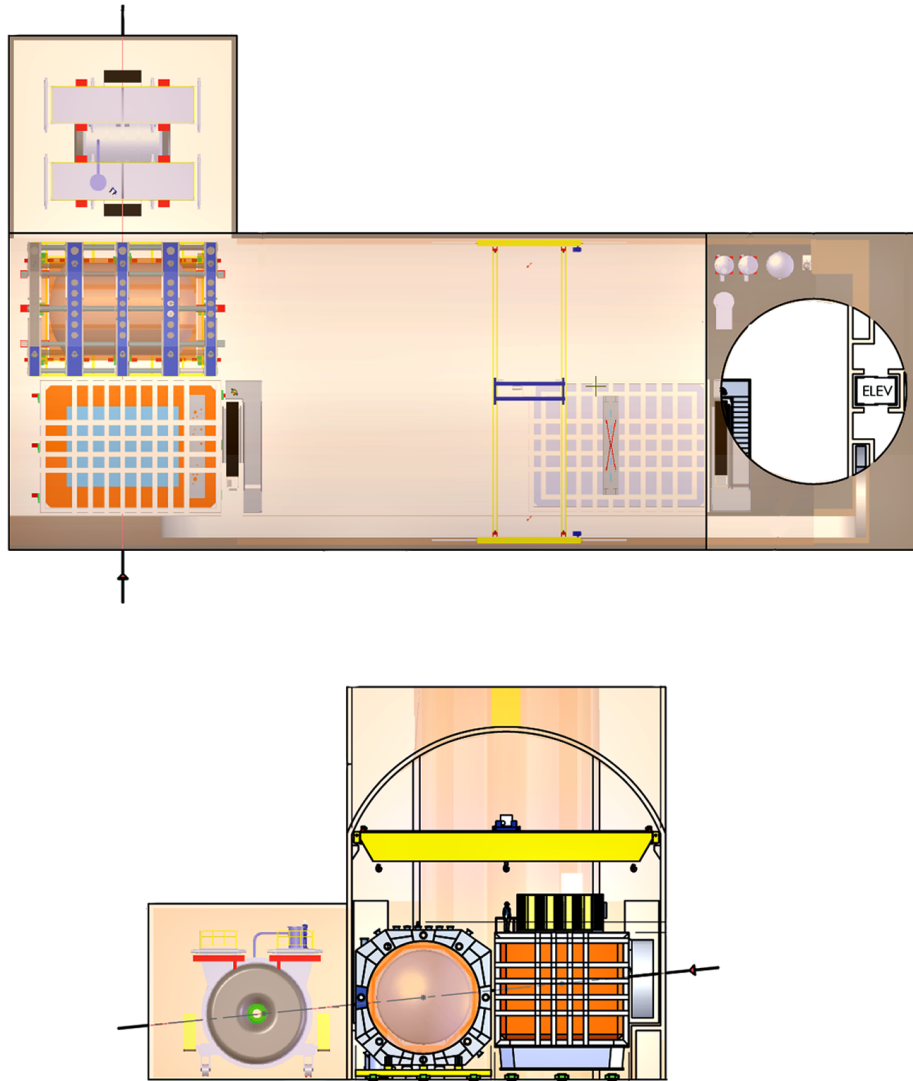
Figure 5.7. DUNE ND hall shown from above (top) and from the side transverse to the beam (bottom). The ArgonCube, MPD and SAND are shown (in that order, bottom to top, in the upper figure) in position on the beam axis (black arrow) in both drawings.
