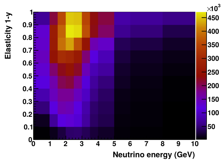
Figure A.9. Events where the visible hadronic system is contained within the nominal 25 t FV , in FHC at 1.07 MW, per year, rates are per bin. The elasticity is the fraction of the original neutrino energy that is carried by the outgoing lepton.
