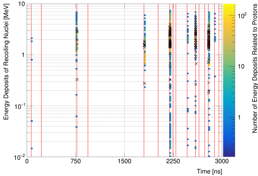
Figure A.14. The temporal distribution of neutrino vertices (red lines) within a beam spill in the LAr component of DUNE ND . The mean separation of neutrino vertices is 279 ns. The filled bins show the number of hits due to recoiling protons, crosses indicate a hit due to a recoiling ^2\text{H} , ^3\text{H} , ^2\text{He} or ^3\text{He} nucleus. All fast-neutron induced energy deposits occur <10 ns after each neutrino interaction.
