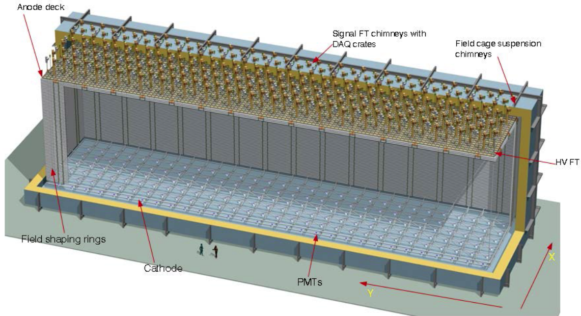
Figure 1.8. Schematic of a 10 kt DUNE FD/DP detector module with cathode, PMTs , FC , and anode plane with SFT chimneys . The drift direction is vertical in the case of a DP module. The scale is indicated by the figures of two people standing in front of the model.
