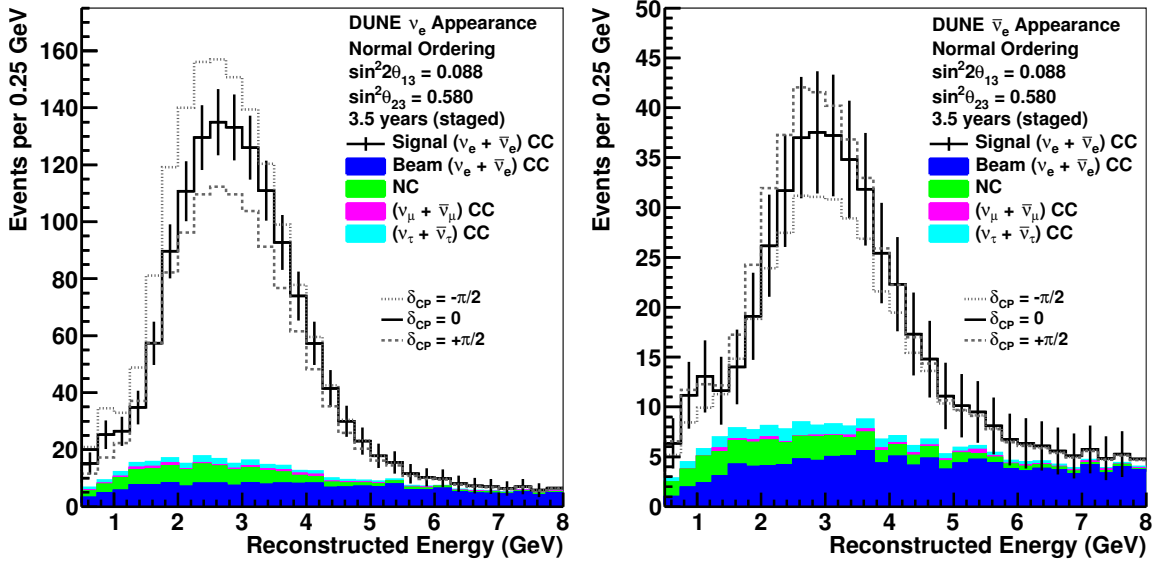
Figure 2.4. \nu_e and \bar{\nu}_e appearance spectra: reconstructed energy distribution of selected \nu_e \overline{\text{CC}} -like events assuming 3.5 years (staged) running in the neutrino-beam mode (left) and antineutrino-beam mode (right), for a total of seven years (staged) exposure. The plots assume normal mass ordering and include curves for \delta_{\text{CP}} = -\pi/2, 0, \text{ and } \pi/2 .
