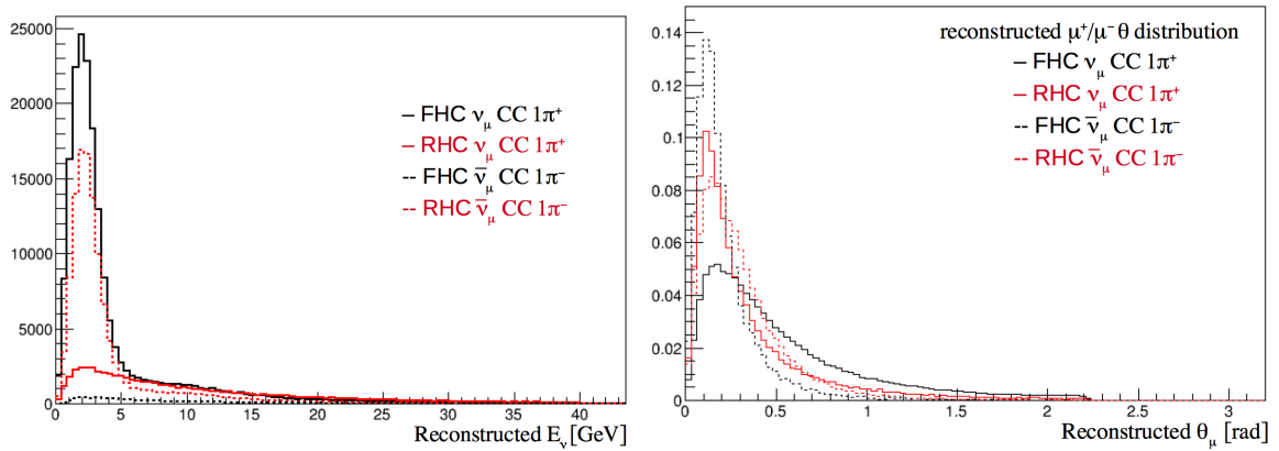
Figure A.17. Representative differences among subsamples of \text{CC } \nu_\mu interactions with one \pi^+ (solid lines) and \text{CC } \bar{\nu}_\mu interactions with one \pi^- (dashed lines). The forward- and reverse- horn current samples are shown in black and red, respectively. Left: reconstructed neutrino energy spectra, normalized to the same number of protons on target. Right: angle of outgoing muon relative to neutrino direction, normalized to unit area for shape comparison.
