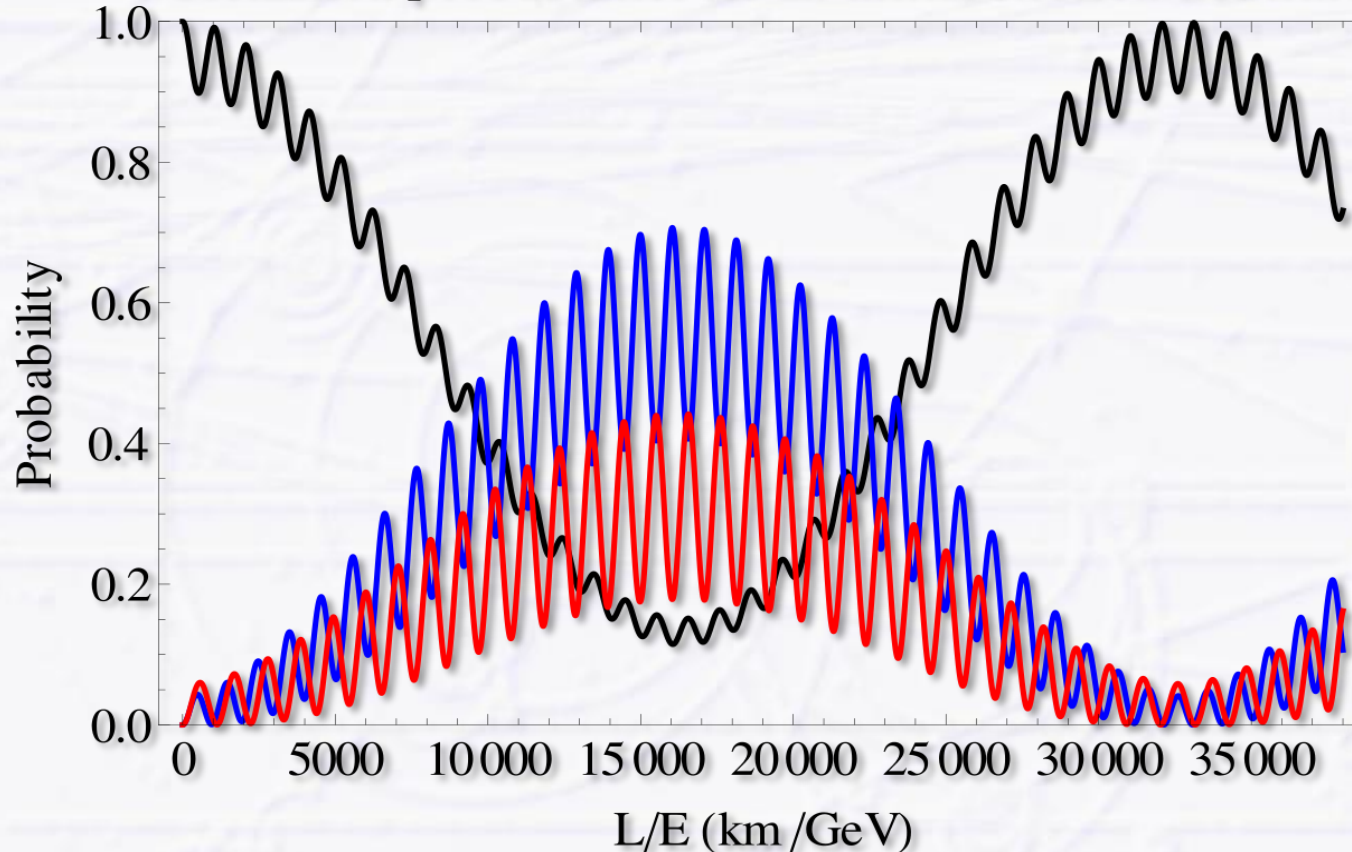
Oscillation probabilities for an initial electron neutrino
