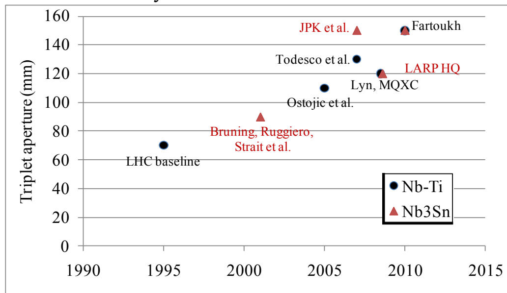
Optimal aperture for the LHC triplet versus time
