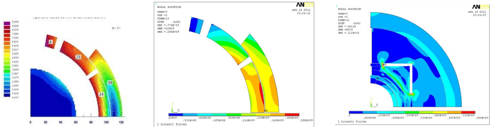
Preliminary study on 180 mm aperture D1 [Q. Xu]
