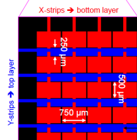
\mu RWELL with capacitive-sharing strip readout
